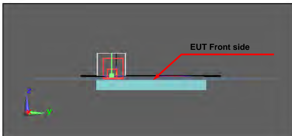
Figure 6. Body SAR Test Setup (Flat Section)
