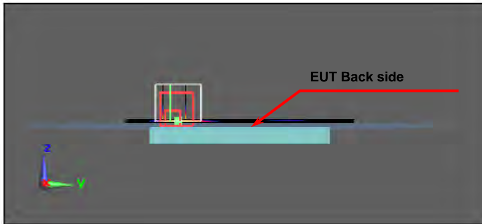
Figure 7. Body SAR Test Setup (Flat Section)
