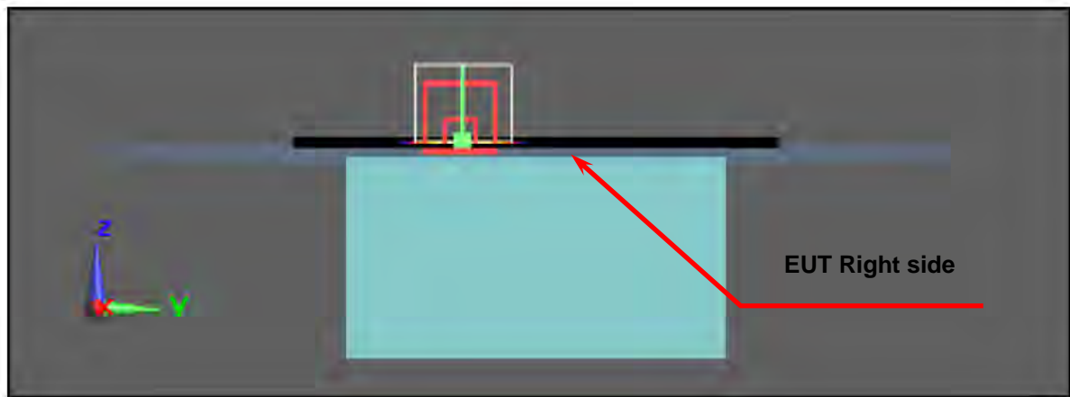
Figure 10. Body SAR Test Setup (Flat Section)
