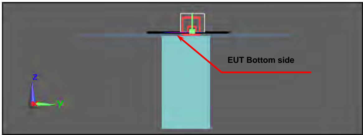
Figure 9. Body SAR Test Setup (Flat Section)
