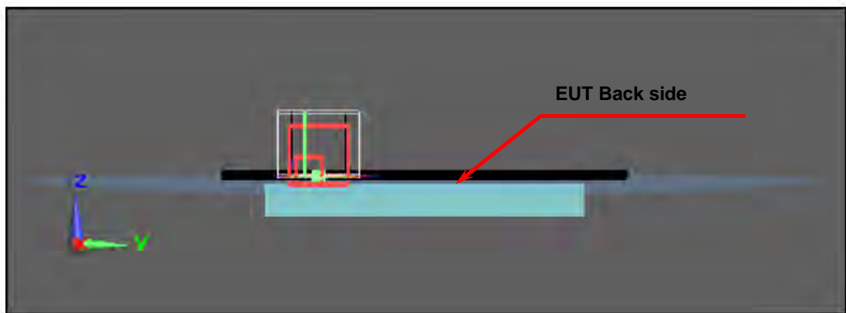
Figure 8. Body SAR Test Setup (Flat Section)
