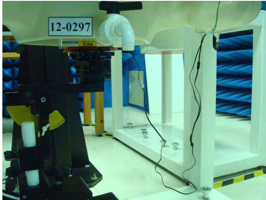
Figure 8. Body SAR Test Setup (Flat Section)
