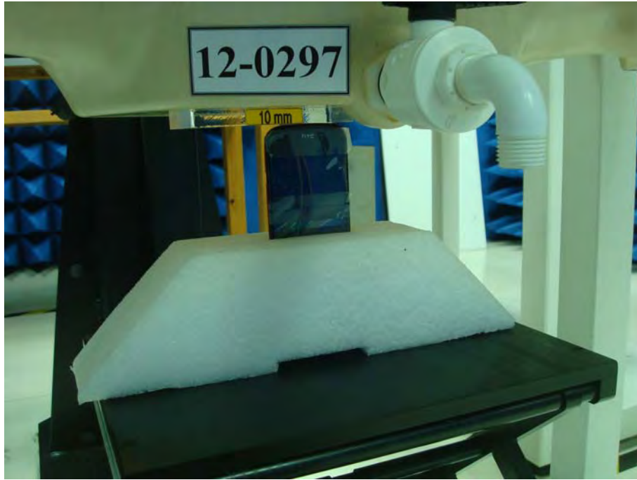
Figure 12. Body SAR Test Setup (Flat Section)
