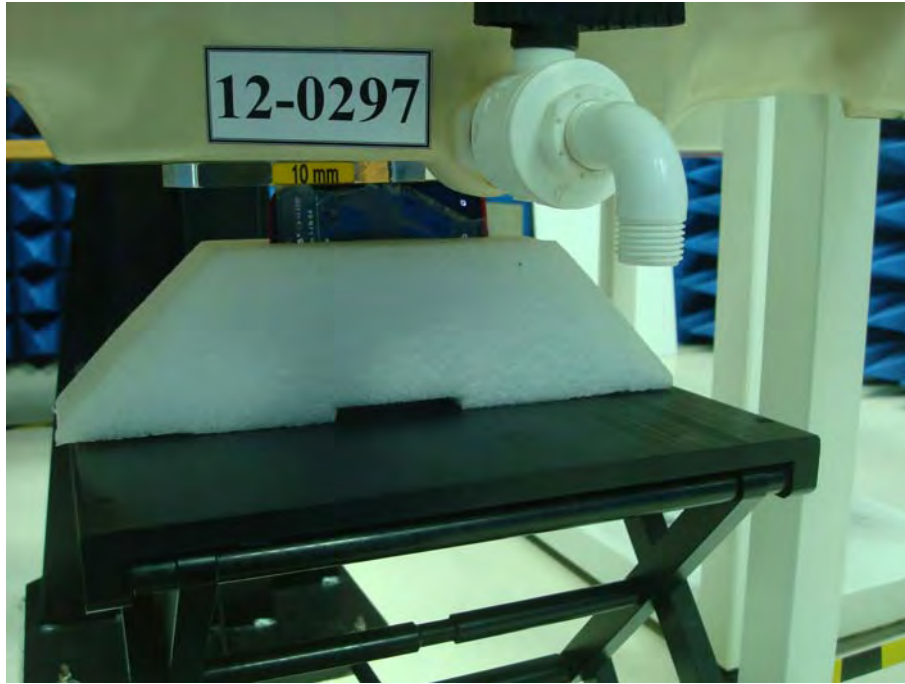
Figure 10. Body SAR Test Setup (Flat Section)
