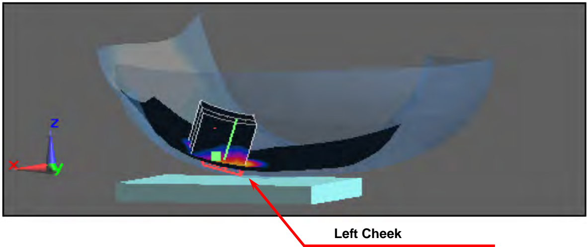
Figure 3. Left Head SAR Test Setup (Cheek)
