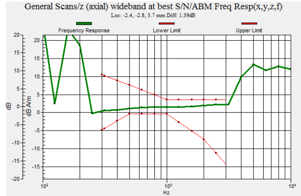
Fig. 9.8 WCDMA Band V Ch4182 for Sample 1
