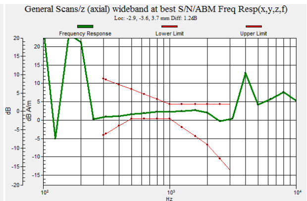
Fig. 9.6 GSM1900 Ch810 for Sample 1
