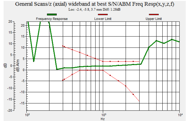
Fig. 9.15 WCDMA Band IV Ch1513 for Sample 1
