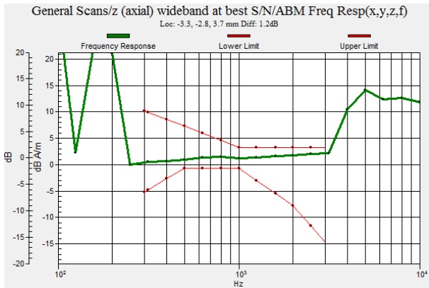
Fig. 9.9 WCDMA Band V Ch4233 for Sample 1
