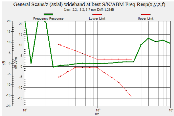
Fig. 9.18 WCDMA Band II Ch9538 for Sample 1
