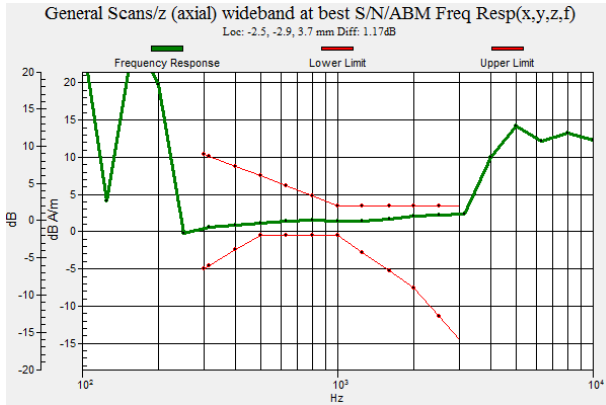
Fig. 9.7 WCDMA Band V Ch4132 for Sample 1
