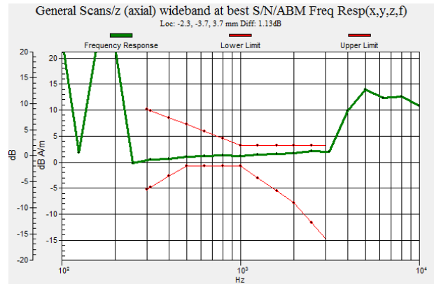
Fig. 9.17 WCDMA Band II Ch9400 for Sample 1
