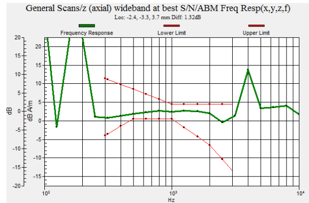
Fig. 9.2 GSM850 Ch189 for Sample 1
