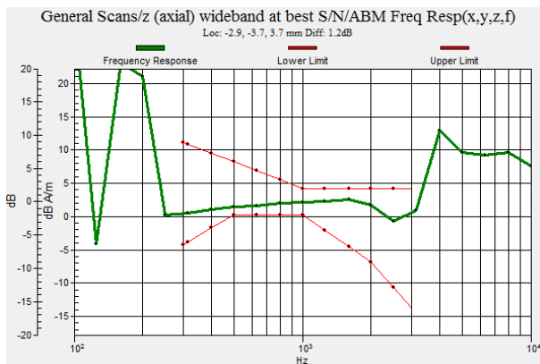
Fig. 9.5 GSM1900 Ch661 for Sample 1
