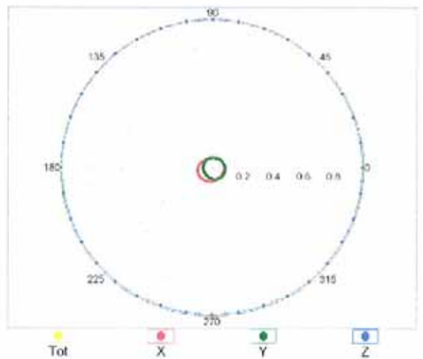
f=2500 MHz,R22,90°
