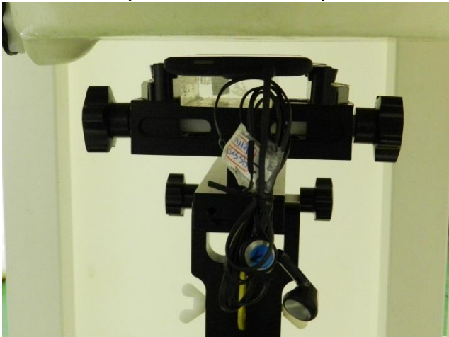
Front of the DUT with Phantom 1 cm Gap (DUT with Headset 2)
