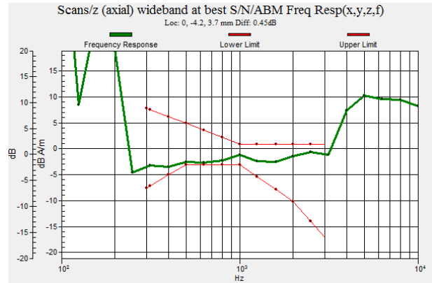
Fig. 9.12 CDMA2000 BC15 Ch875 (Sample 2)
