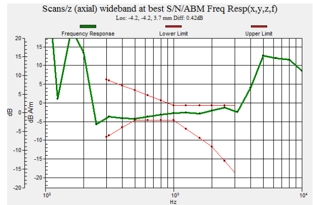
Fig. 9.4 CDMA2000 BC0 Ch1013 (Sample 2)
