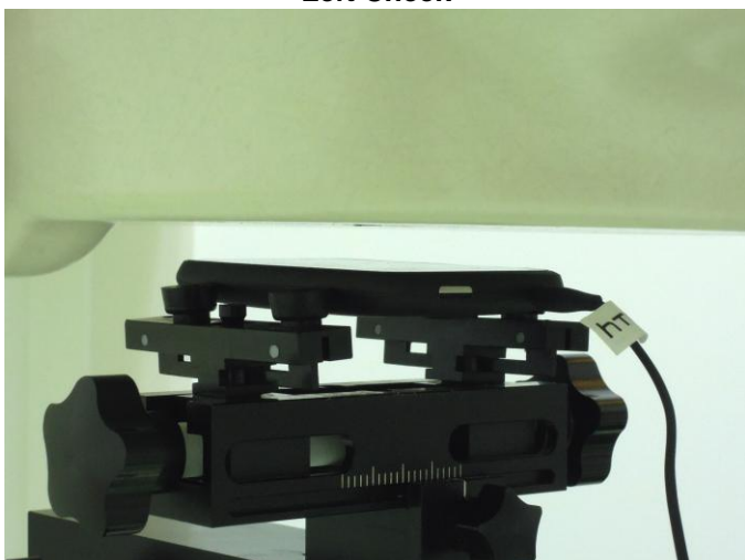
Front Face of DUT with 1 cm Gap (Body-Worn Mode)
