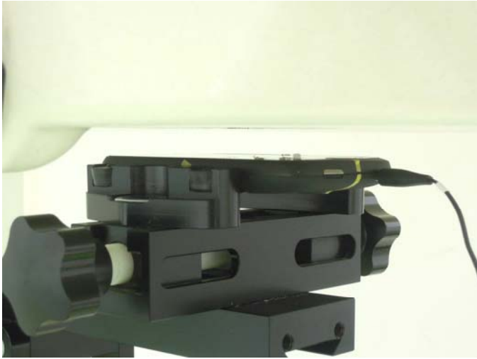
Front Face of DUT with 1 cm Gap (Body Worn, EUT + Earphone 1)
