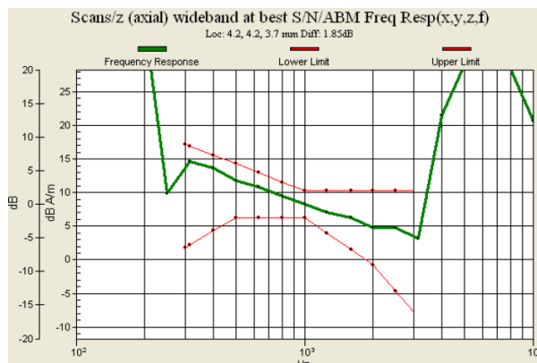
Fig. 9.4 CDMA2000 BC0 Ch777 (Sample 2)
