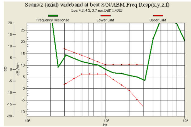
Fig. 9.8 CDMA2000 BC1 Ch600 (Sample 2)
