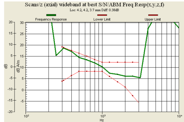
Fig. 9.10 CDMA2000 BC15 Ch425 (Sample 1)
