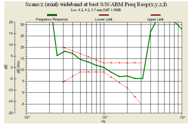
Fig. 9.12 CDMA2000 BC15 Ch25 (Sample 2)
