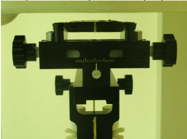
Back of the DUT with Phantom 1 cm Gap (DUT without Earphone for Sample 1)
