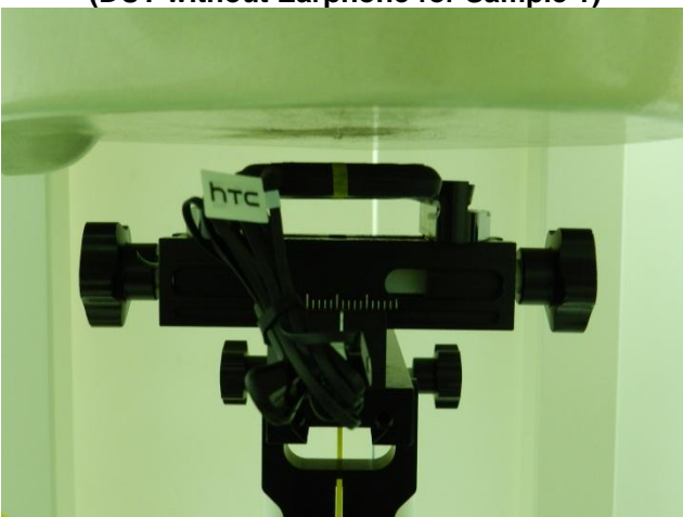
Back of the DUT with Phantom 1 cm Gap (DUT with Earphone for Sample 1)
