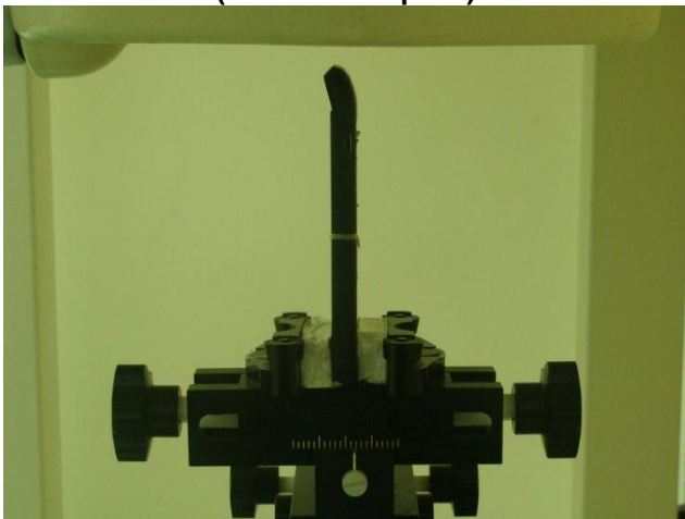
Bottom Side of the DUT with Phantom 1 cm Gap (DUT for Sample 1)
