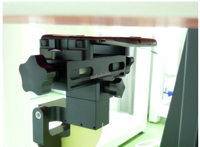
Rear Face of EUT with 1 cm Gap (EUT without Earphone)
