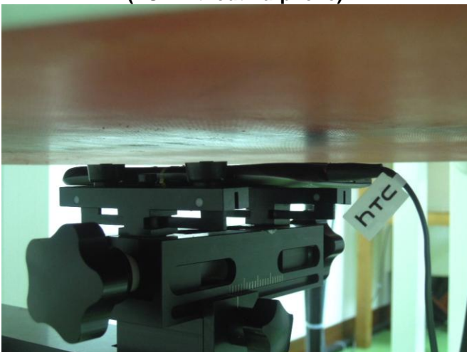
Front Face of EUT with 1 cm Gap (EUT with Earphone)
