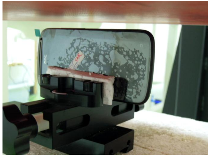
Right Side of EUT with 1 cm Gap (EUT without Earphone)
