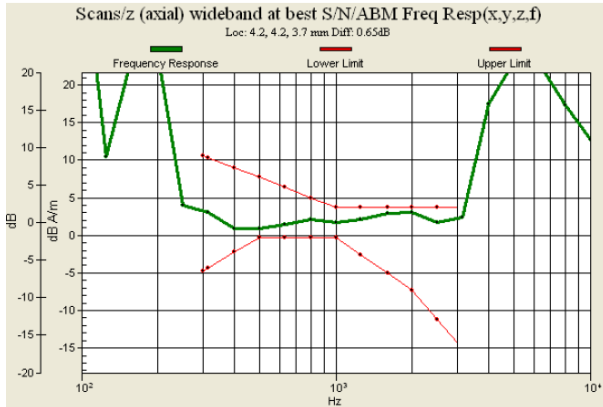
Fig. 9.13 WCDMA Band II Ch9262 (DUT for Sample 1)
