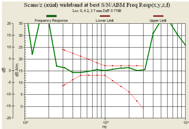
Fig. 9.15 WCDMA Band II Ch9538 (DUT with Battery 1 for Sample 1)
