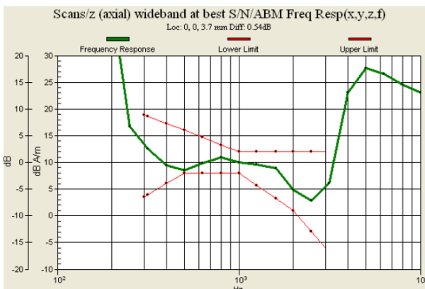
Fig. 9.5 GSM1900 Ch512 (DUT for Sample 1)
