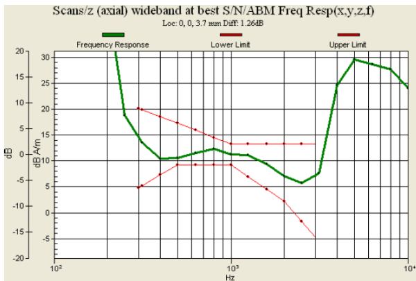
Fig. 9.3 GSM850 Ch251 (DUT for Sample 1)
