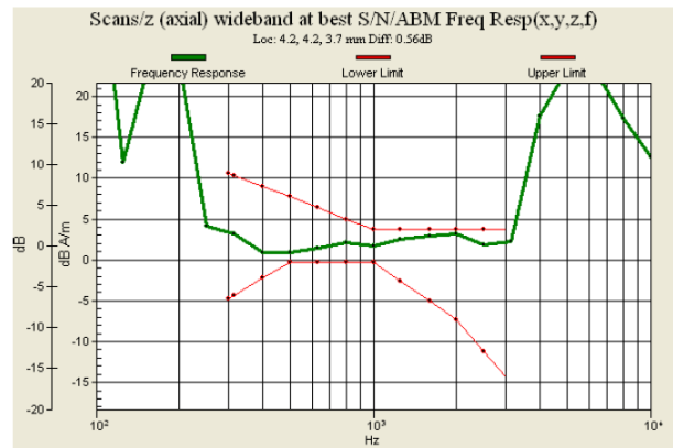
Fig. 9.14 WCDMA Band II Ch9400 (DUT for Sample 1)
