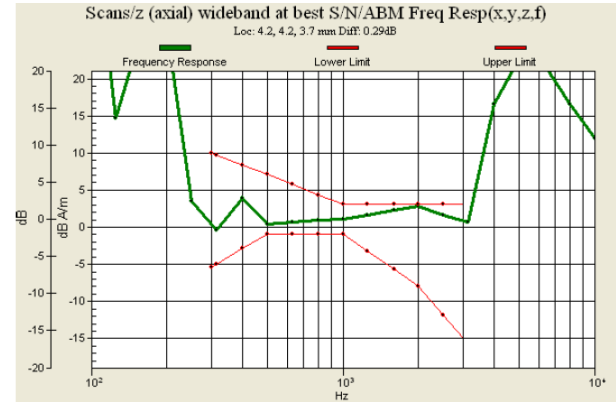
Fig. 9.10 WCDMA Band V Ch4182 (DUT for Sample 1)
