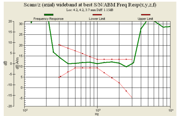
Fig. 9.12 WCDMA Band V Ch4132 (DUT for Sample 2)
