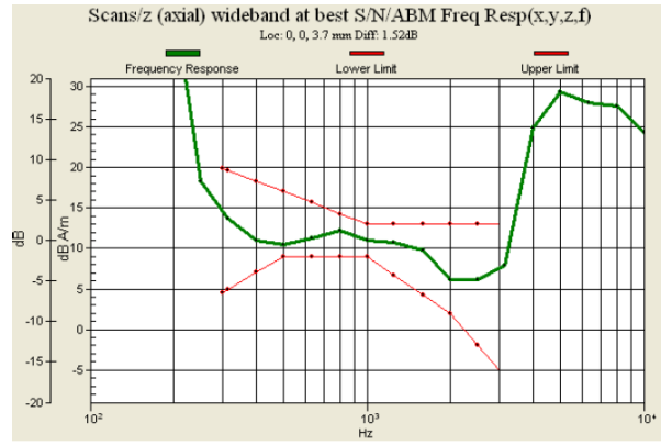
Fig. 9.2 GSM850 Ch189 (DUT for Sample 1)
