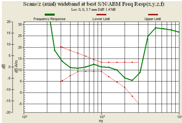
Fig. 9.7 GSM1900 Ch810 (DUT for Sample 1)
