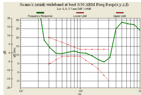
Fig. 9.6 GSM1900 Ch661 (DUT for Sample 1)
