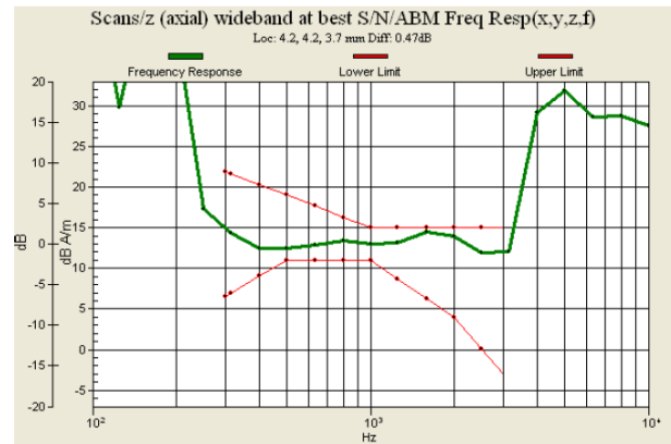
Fig. 9.8 GSM1900 Ch512 (DUT for Sample 2)
