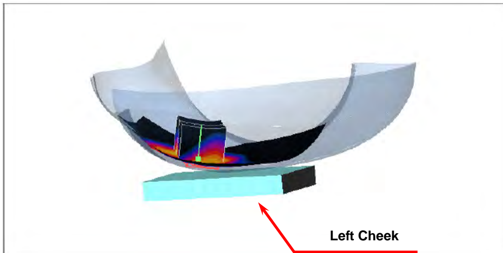
Figure 3. Left Head SAR Test Setup (Cheek)
