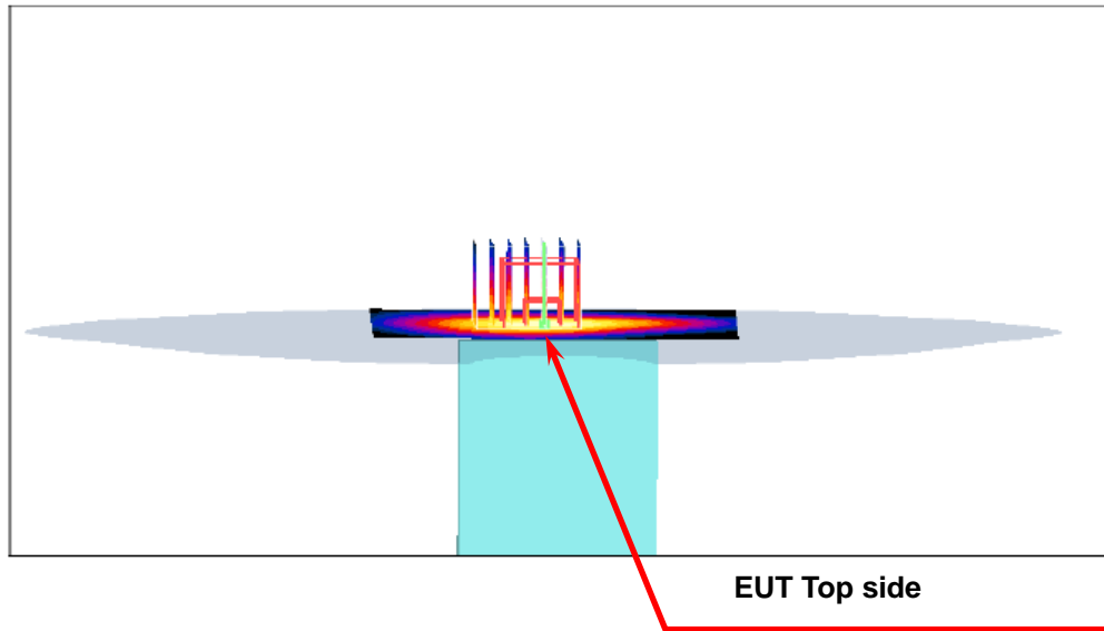
Figure 10. Body SAR Test Setup (Flat Section)
