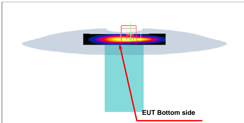
Figure 9. Body SAR Test Setup (Flat Section)
