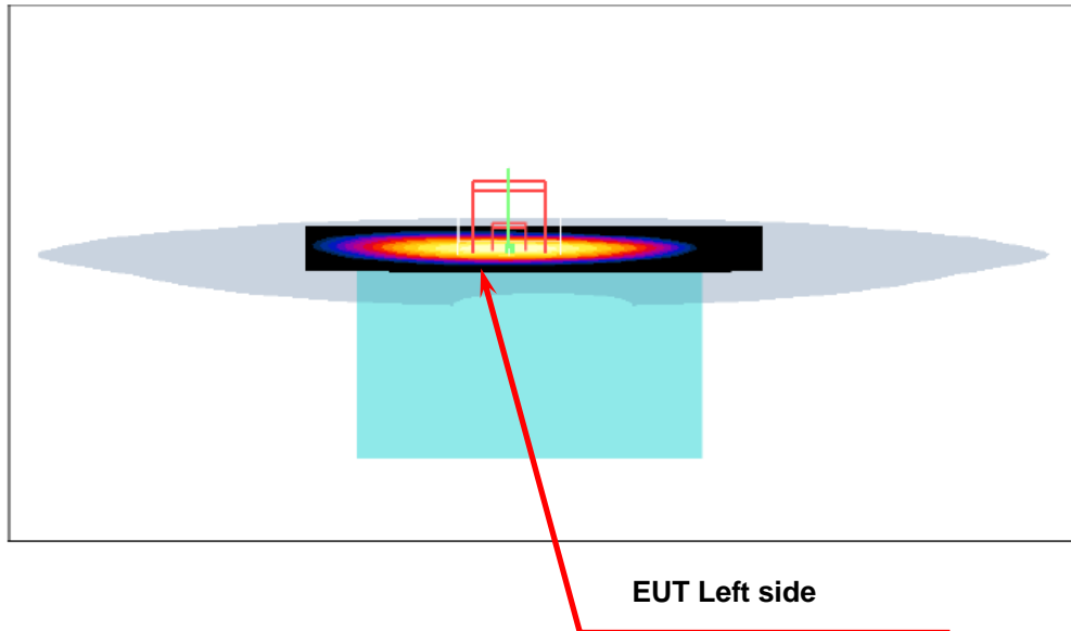
Figure 8. Body SAR Test Setup (Flat Section)
