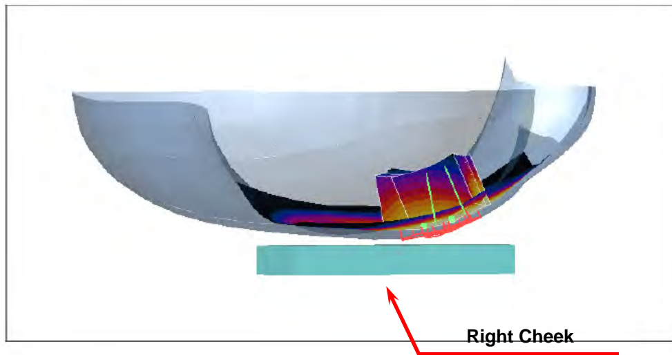
Figure 1. Right Head SAR Test Setup (Cheek)
