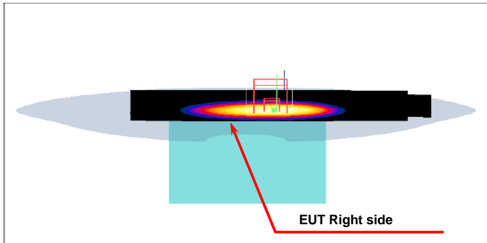
Figure 7. Body SAR Test Setup (Flat Section)
