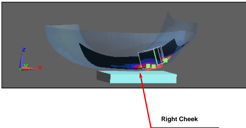
Figure 1. Right Head SAR Test Setup (Cheek)
