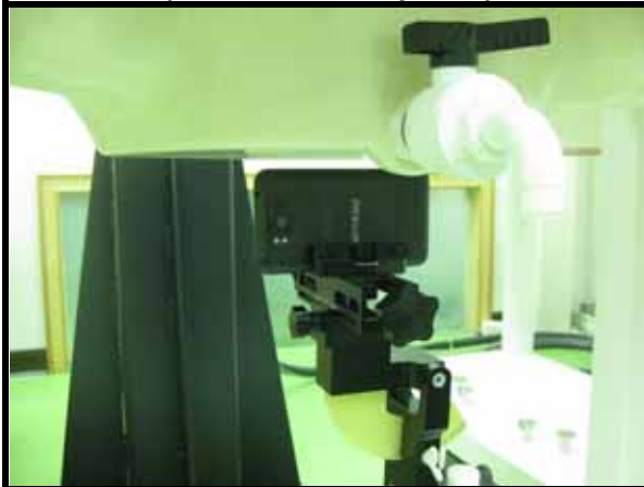
Left Edge with 1 cm Gap (DUT without Earphone)
