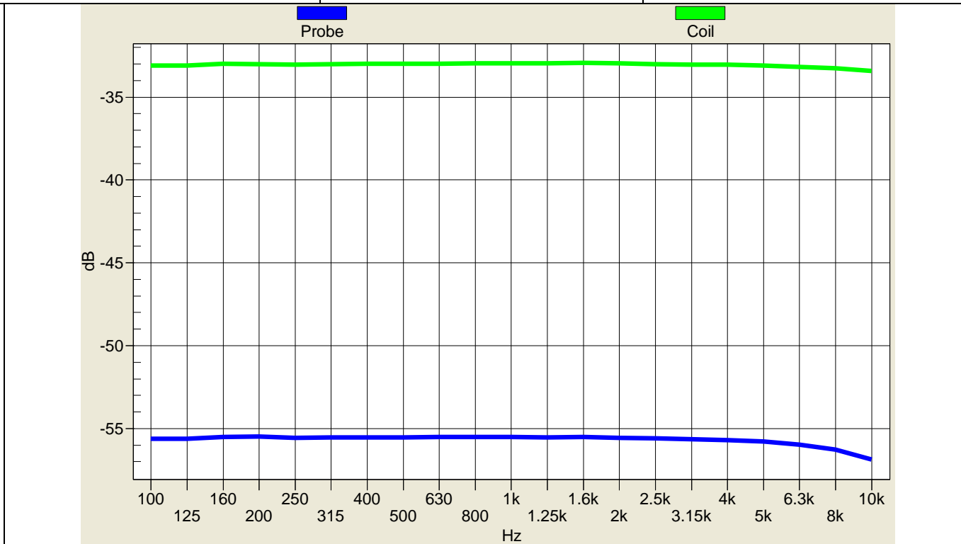
Appendix A1 : The frequency response and sensitivity of AM1D probe
