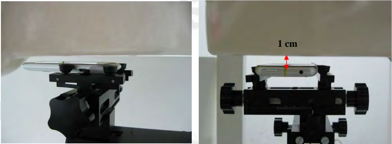
Fig.7 Hotspot mode- EUT front to flat phantom and distance between flat phantom and mobile phone is 1 cm.
