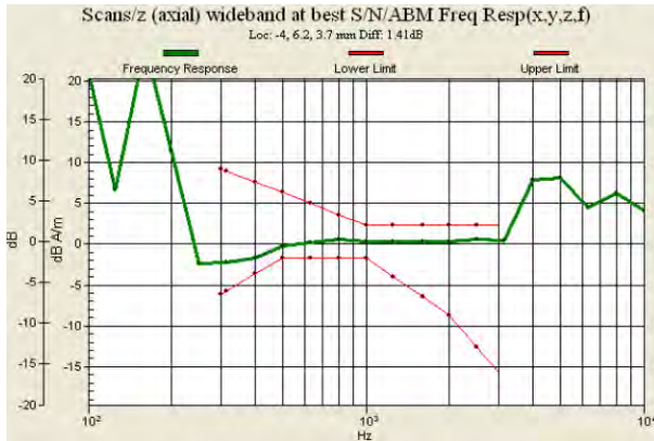
Fig. 9.13 WCDMA Band IV Ch1312 (DUT with Battery 1 for Sample 1)
