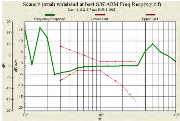
Fig. 9.19 WCDMA Band II Ch9538 (DUT with Battery 1 for Sample 1)
