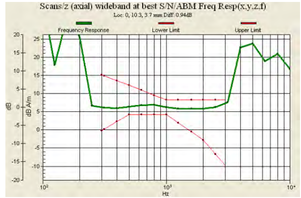
Fig. 9.20 WCDMA Band II Ch9262 (DUT with Battery 2 for Sample 2)
