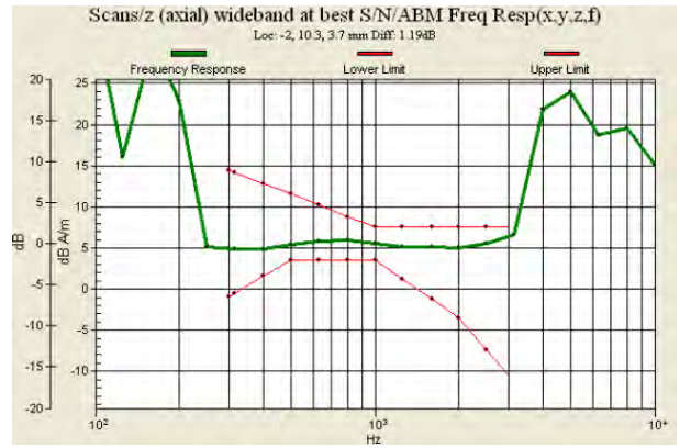
Fig. 9.16 WCDMA Band IV Ch1513 (DUT with Battery 2 for Sample 2)
