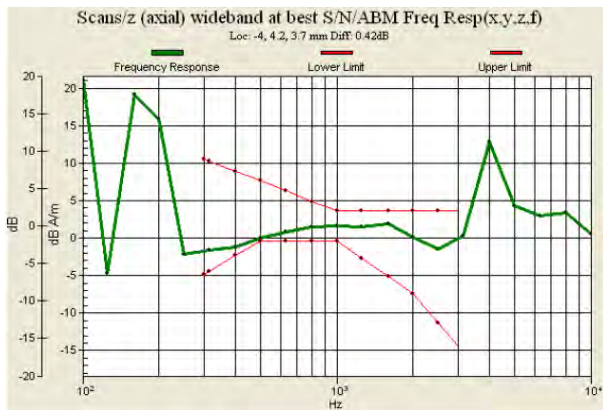
Fig. 9.5 GSM1900 Ch512
