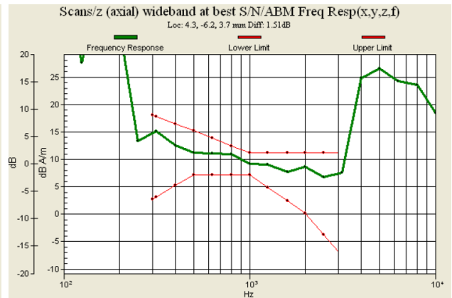
Fig. 9.4 CDMA2000 BC0 Ch1013 (DUT with Battery 2)
