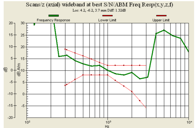
Fig. 9.6 CDMA2000 BC1 Ch600 (DUT with Battery 1)
