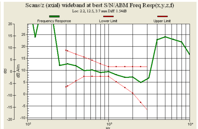
Fig. 9.10 CDMA2000 BC10 Ch476 (DUT with Battery 2)
