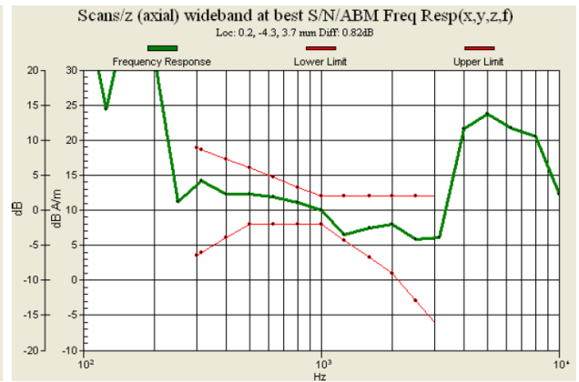
Fig. 9.2 CDMA2000 BC0 Ch384 (DUT with Battery 1)
