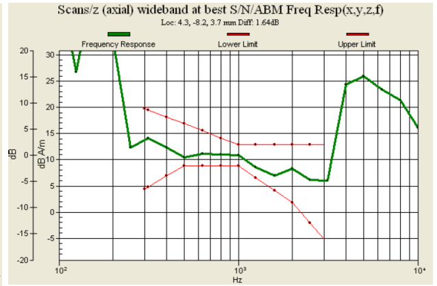
Fig. 9.8 CDMA2000 BC1 Ch1175 (DUT with Battery 2)
