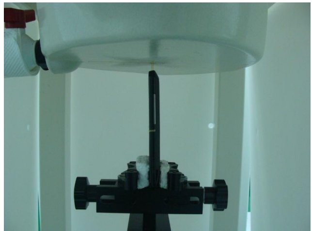
Top Side of the DUT with Phantom 1 cm Gap for DUT without Earphone
