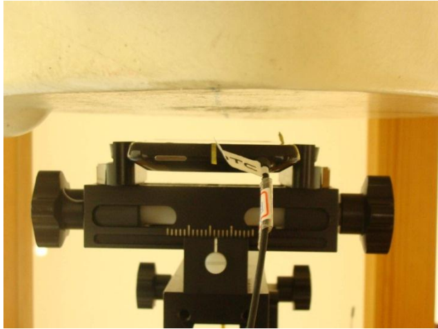
Front of the DUT with Phantom 1 cm Gap for DUT with Earphone 2
