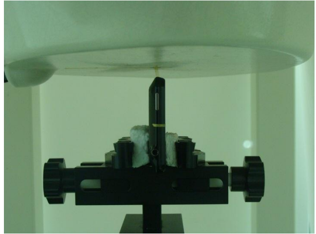
Right Side of the DUT with Phantom 1 cm Gap for DUT without Earphone
