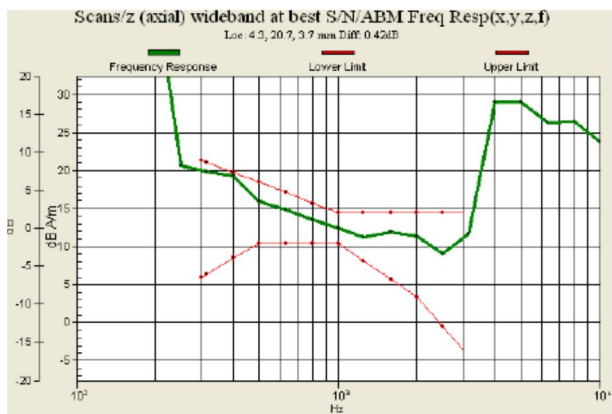
Fig. 9.4 GSM1900 Ch512 with Battery 1
