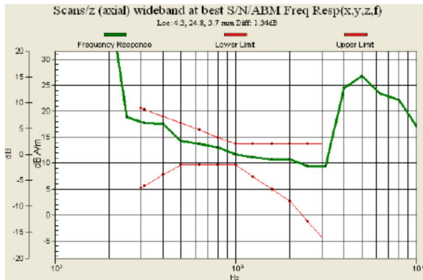
Fig. 9.1 GSM850 Ch128 with Battery 1
