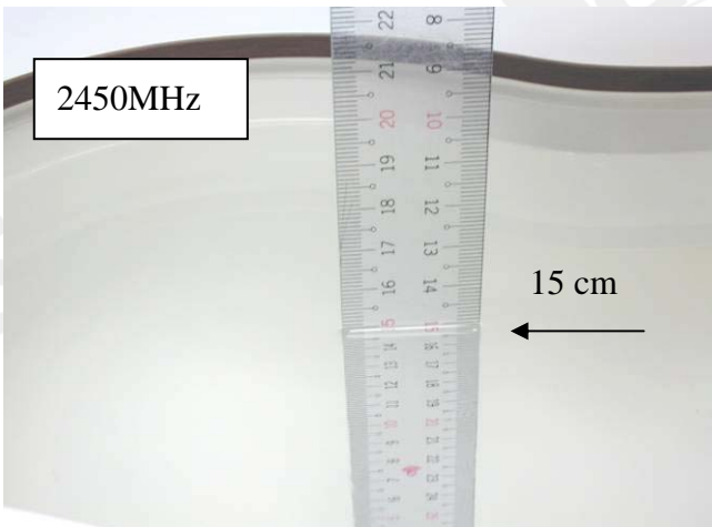
Fig.2.5 Photograph of the Tissue Simulant Fluid liquid depth 15cm for Right-head Side
