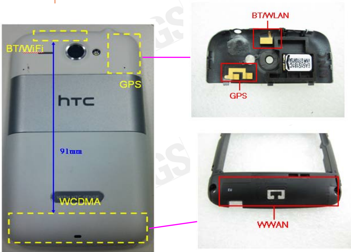
Fig.17 Antenna position & Antenna distance
