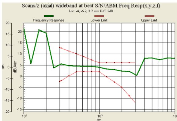
Fig. 9.9 CDMA2000 BC10 Ch476 (DUT with Battery 1)
