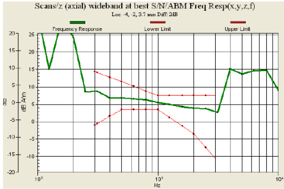
Fig. 9.5 CDMA2000 BC1 Ch25 (DUT with Battery 1)
