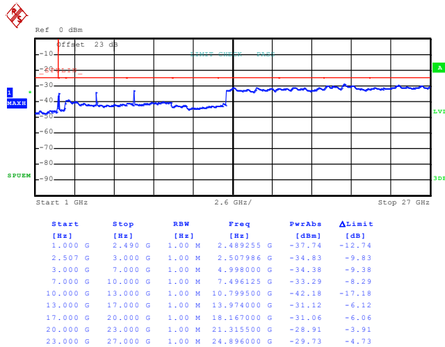
Conducted Spurious Emission Plot between 1GHz ~ 27GHz
