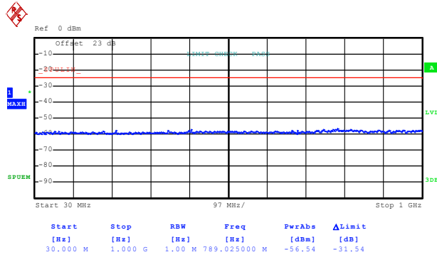
Conducted Spurious Emission Plot between 30MHz ~ 1GHz
