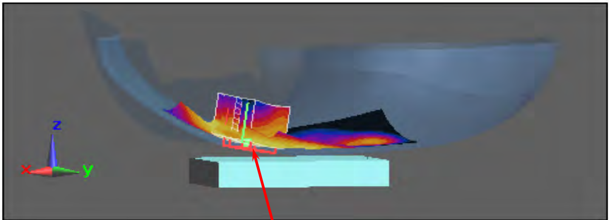
Figure 3. Left Head SAR Test Setup (Cheek)
