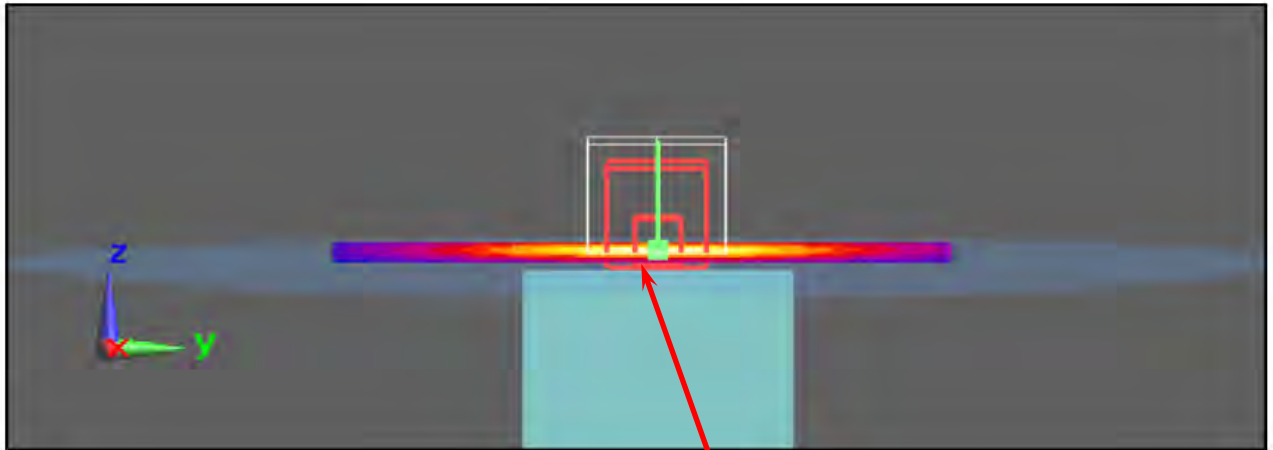
Figure 9. Body SAR Test Setup (Flat Section)
