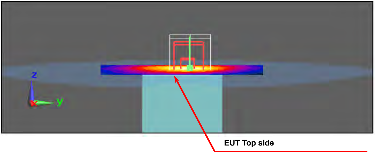
Figure 10. Body SAR Test Setup (Flat Section)
