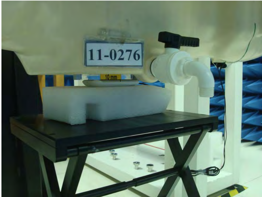
Body Setup _ Front Surface to Phantom 10mm (EUT with Headset)
