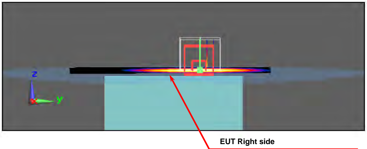
Figure 8. Body SAR Test Setup (Flat Section)
