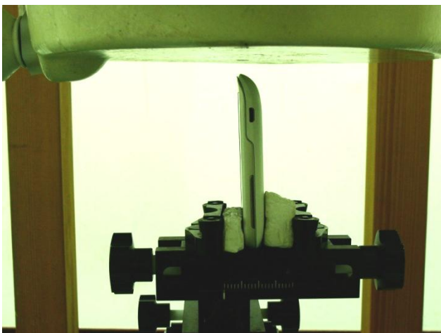
Bottom of the DUT with Phantom 1 cm Gap (DUT without Earphone)
