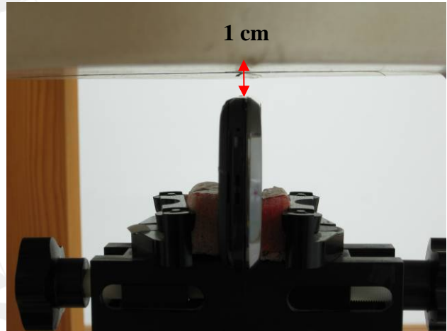
Fig.16 Hotspot mode - EUT Left to flat phantom and distance between flat phantom and mobile phone is 1 cm.
