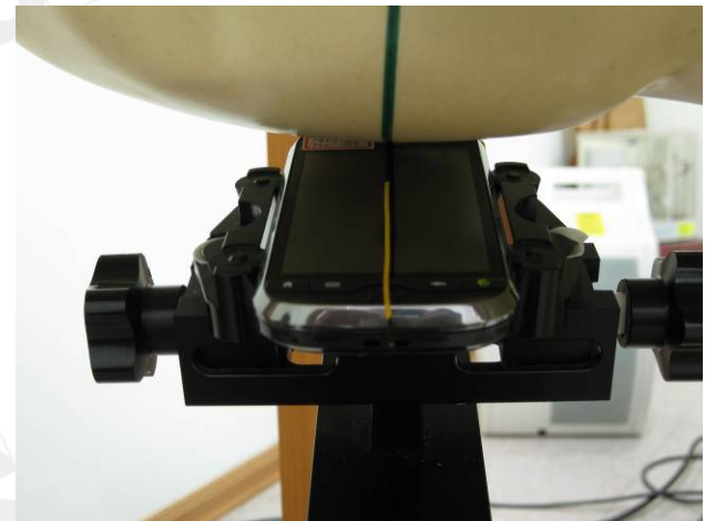
Fig.4 Right Head Section / Ear-Tilt Position(15°)_ Slider off
