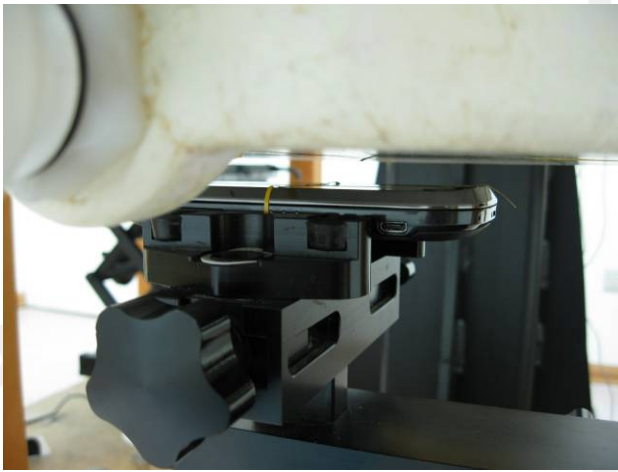
Fig.11 Hotspot mode - EUT front to flat phantom and distance between flat phantom and mobile phone is 1 cm.
