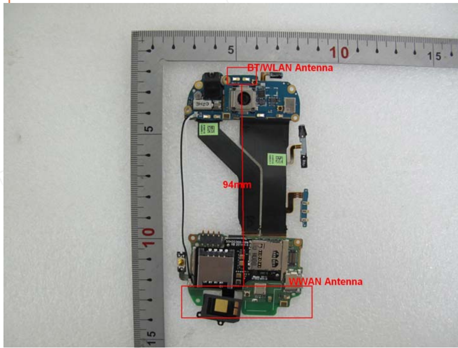
Fig.31 Antenna position of EUT
