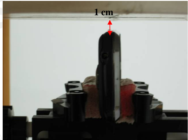
Fig.15 Hotspot mode - EUT Right to flat phantom and distance between flat phantom and mobile phone is 1 cm.
