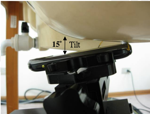
Fig.6 Left Head Section / Ear-Tilt Position(15°)_ Slider off
