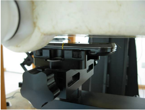
Fig.11 Hotspot mode - EUT front to flat phantom and distance between flat phantom and mobile phone is 1 cm.
