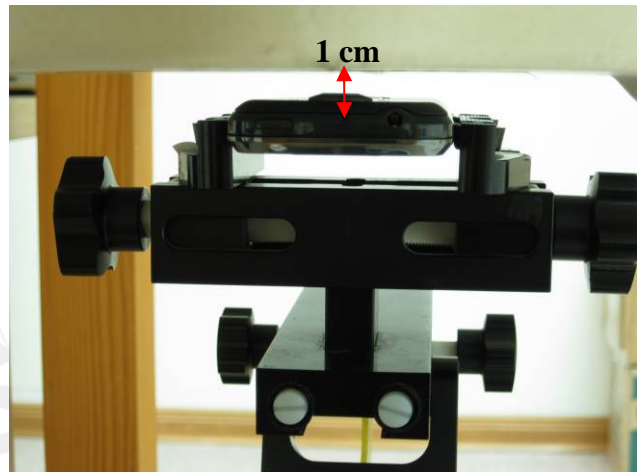
Fig.12 Hotspot mode - EUT back to flat phantom and distance between flat phantom and mobile phone is 1 cm.
