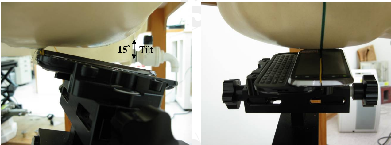
Fig.8 Right Head Section / Ear-Tilt Position(15°)_ Slider on
