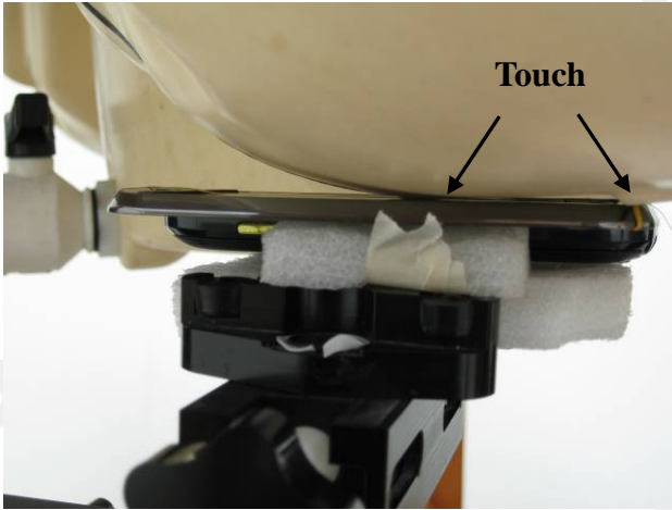
Fig.9 Left Head Section / Cheek-Touch Position_ Slider on
