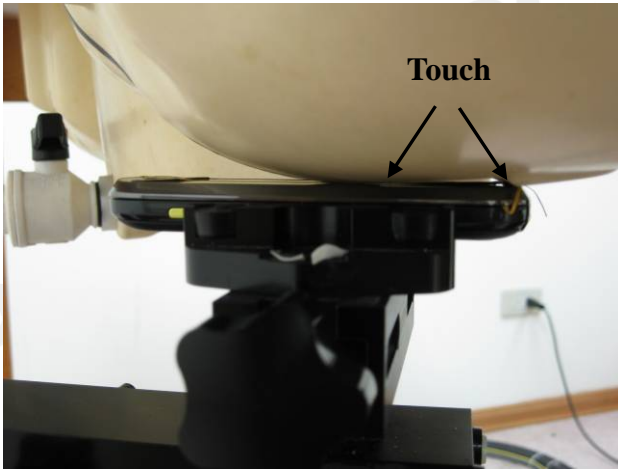
Fig.5 Left Head Section / Cheek-Touch Position_ Slider off
