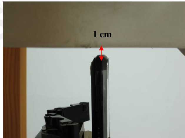
Fig.13 Hotspot mode - EUT Top to flat phantom and distance between flat phantom and mobile phone is 1 cm.
