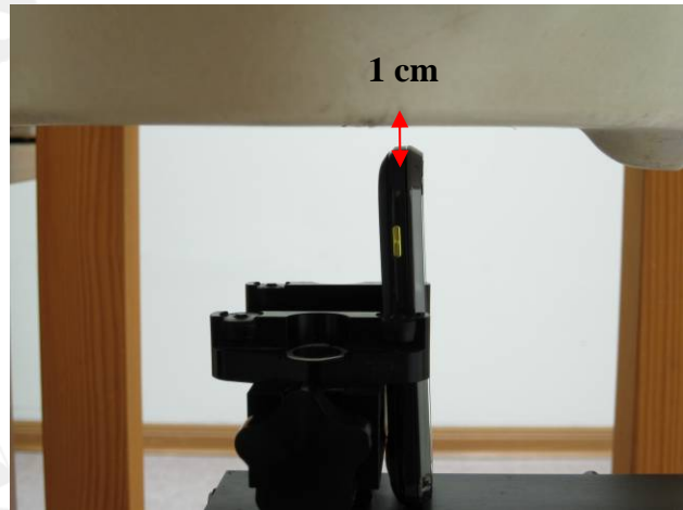
Fig.14 Hotspot mode - EUT Bottom to flat phantom and distance between flat phantom and mobile phone is 1 cm.
