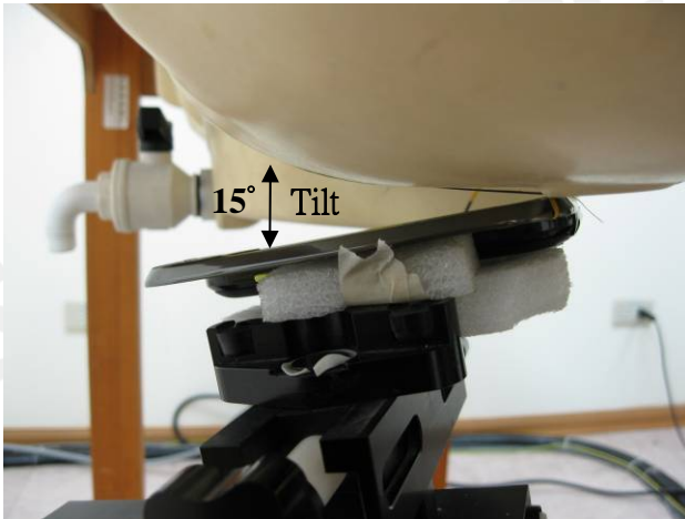
Fig.10 Left Head Section / Ear-Tilt Position(15°)_ Slider on
