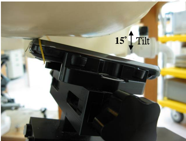
Fig.4 Right Head Section / Ear-Tilt Position(15°)_ Slider off
