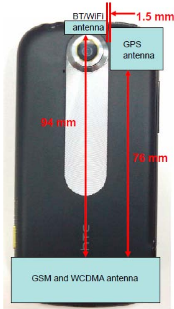
Fig.31 Antenna position of EUT
