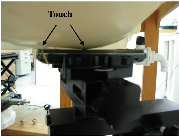
Fig.3 Right Head Section / Cheek-Touch Position_ Slider off
