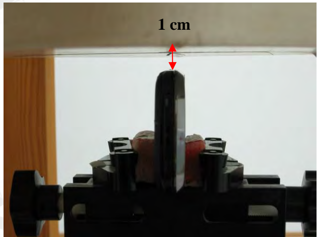
Fig.16 Body worn- EUT Left to flat phantom and distance between flat phantom and mobile phone is 1 cm.
