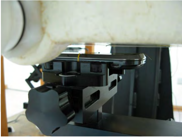
Fig.11 Body worn- EUT front to flat phantom and distance between flat phantom and mobile phone is 1 cm.
