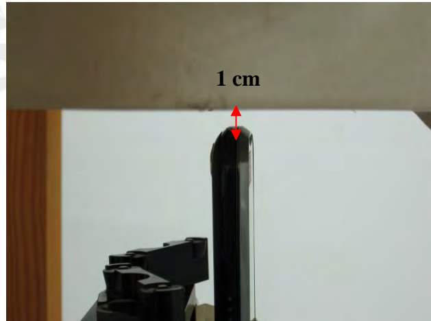
Fig.13 Body worn- EUT Top to flat phantom and distance between flat phantom and mobile phone is 1 cm.
