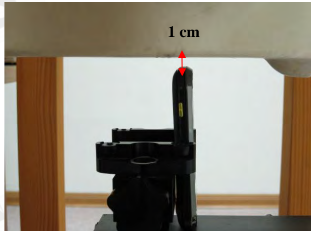
Fig.14 Body worn- EUT Bottom to flat phantom and distance between flat phantom and mobile phone is 1 cm.
