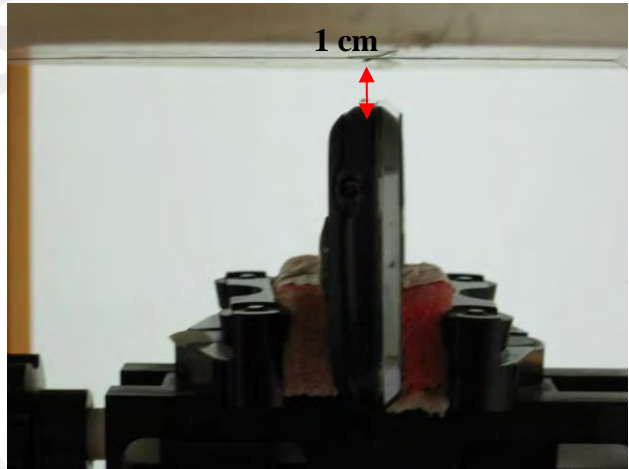
Fig.15 Body worn- EUT Right to flat phantom and distance between flat phantom and mobile phone is 1 cm.
