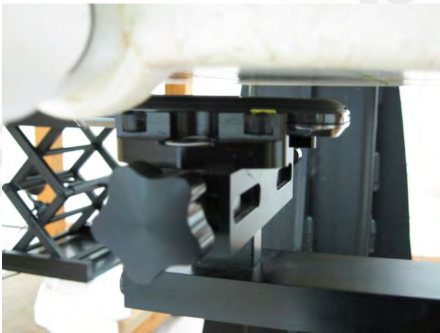
Fig.12 Body worn- EUT back to flat phantom and distance between flat phantom and mobile phone is 1 cm.
