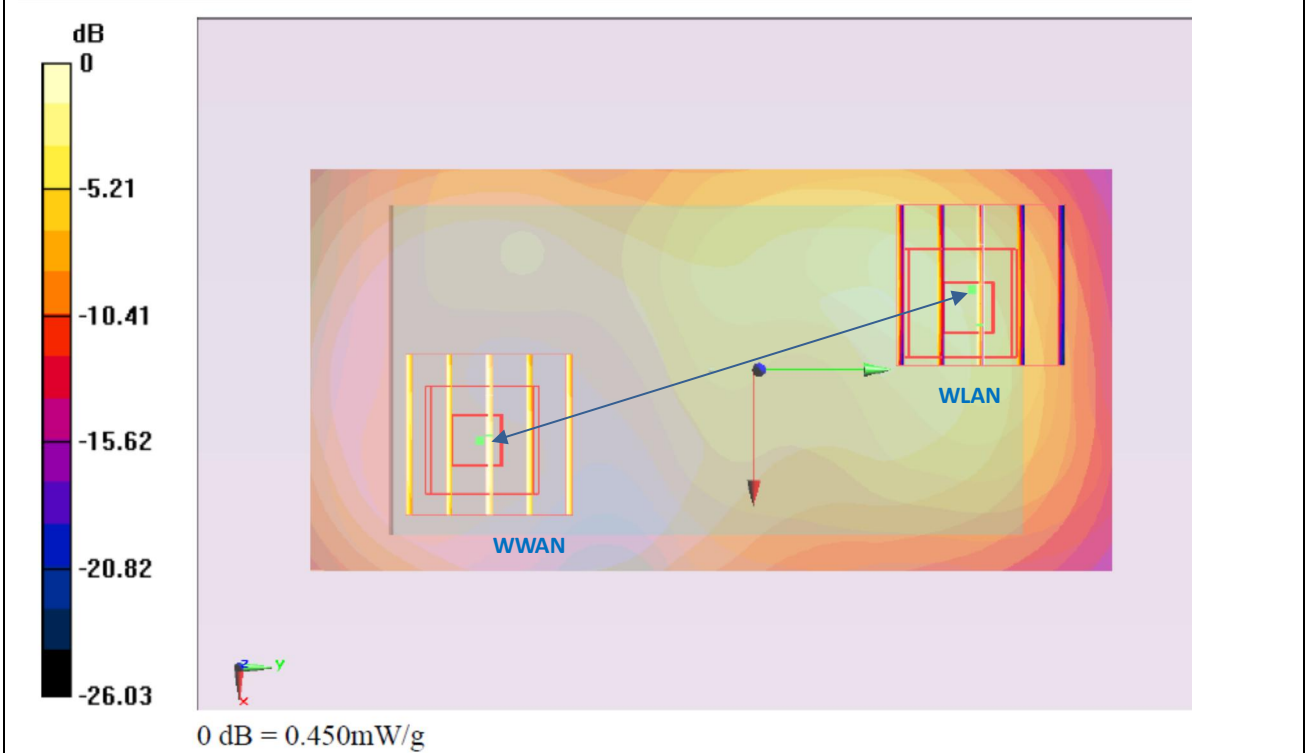
Body- Back, WCDMA Band IV CH1312 + WLAN CH6
