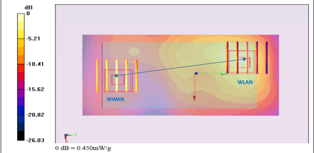
Body- Back, GSM1900 CH661 + WLAN CH6
