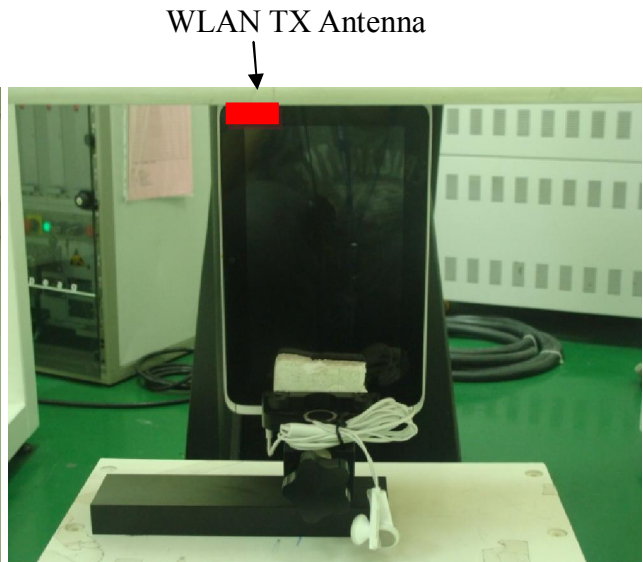
Bottom side, with 0cm to the phantom
