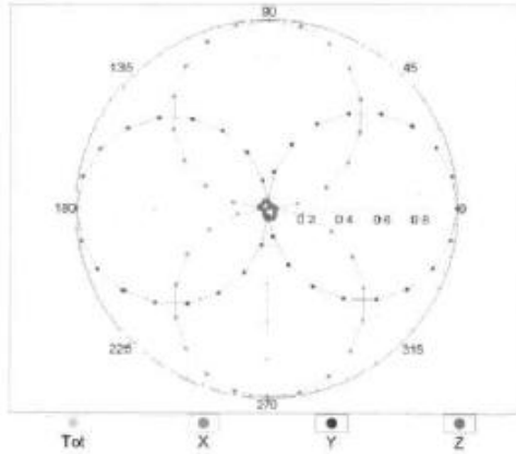
f=600 MHz,TEM,0°
