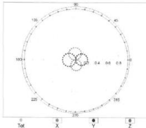
f=2500 MHz,R22,90°
