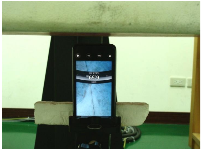
Bottom Side of the DUT with Phantom 1.0 cm Gap for DUT Slide Off Mode without Earphone
