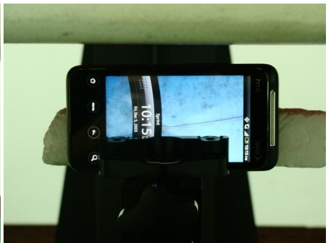
Left Side of the DUT with Phantom 1.0 cm Gap for DUT Slide Off Mode without Earphone
