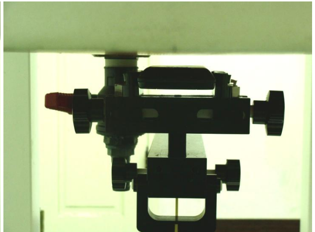
Rear Face of the DUT with Phantom 1.0 cm Gap for DUT Slide Off Mode without Earphone
