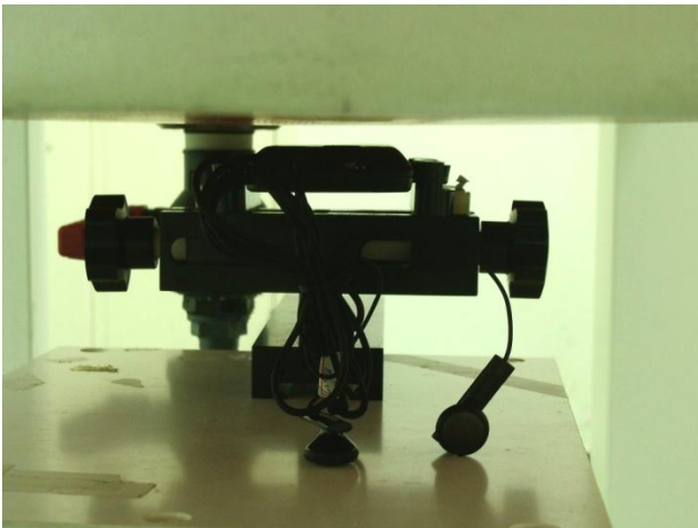
Rear Face of the DUT with Phantom 1.0 cm Gap for DUT Slide Off Mode with Earphone
