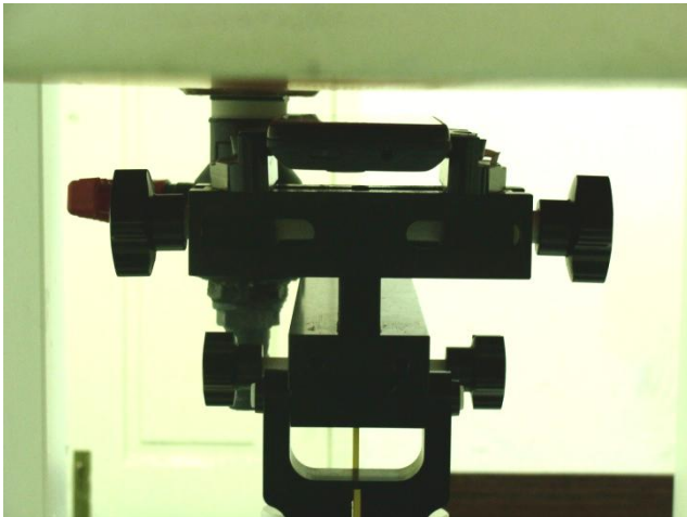
Front Face of the DUT with Phantom 1.0 cm Gap for DUT Slide Off Mode without Earphone
