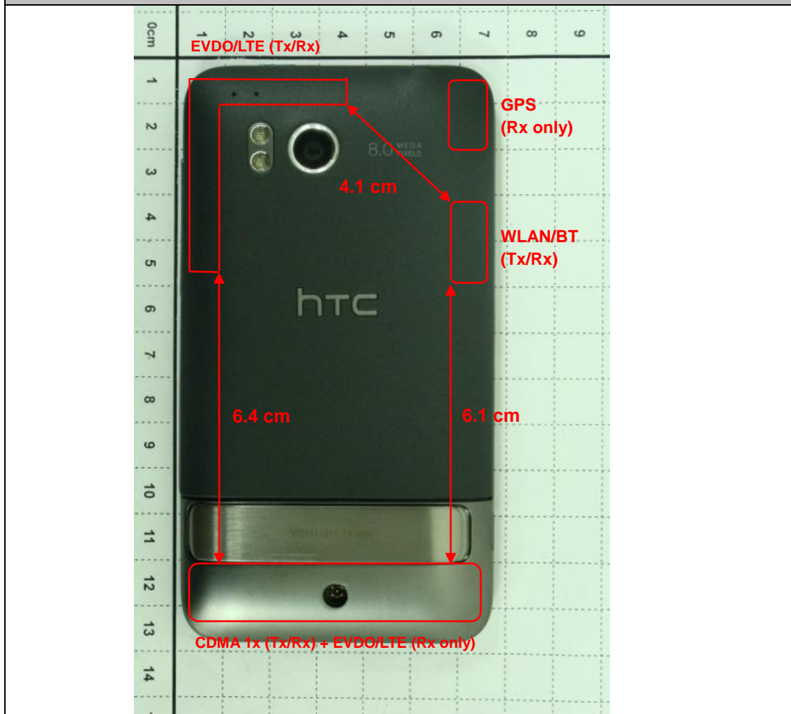
Antenna Location (DUT Rear View)
