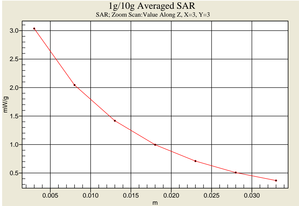
Body-Tissue-Simulating-Liquid 835MHz(02/21/2011)
