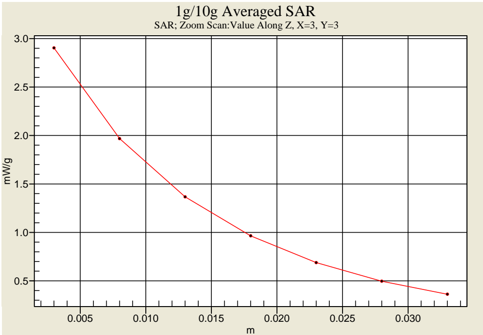
Body-Tissue-Simulating-Liquid 835MHz(11/19/2010)
