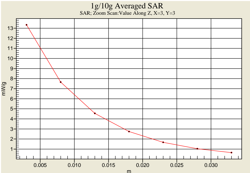
Body-Tissue-Simulating-Liquid 1900MHz(11/19/2010)
