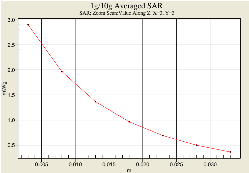
Body-Tissue-Simulating-Liquid 835MHz(09/02/2010)
