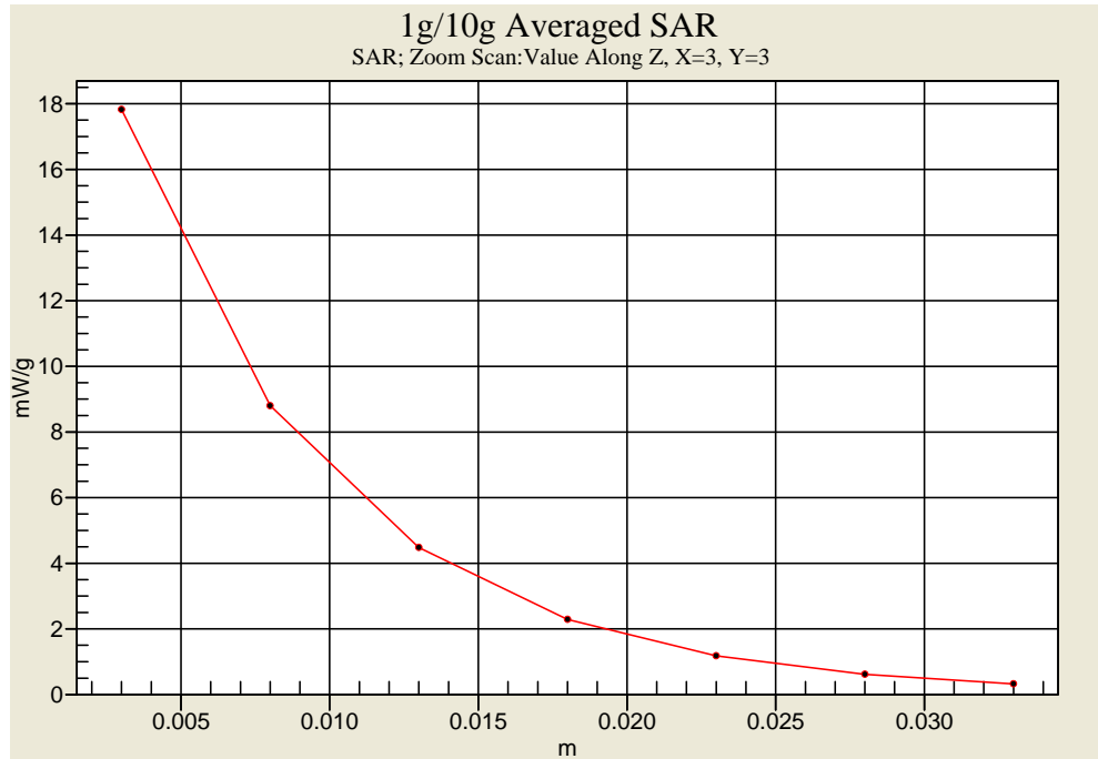
Body-Tissue-Simulating-Liquid 2450MHz(02/22/2011)
