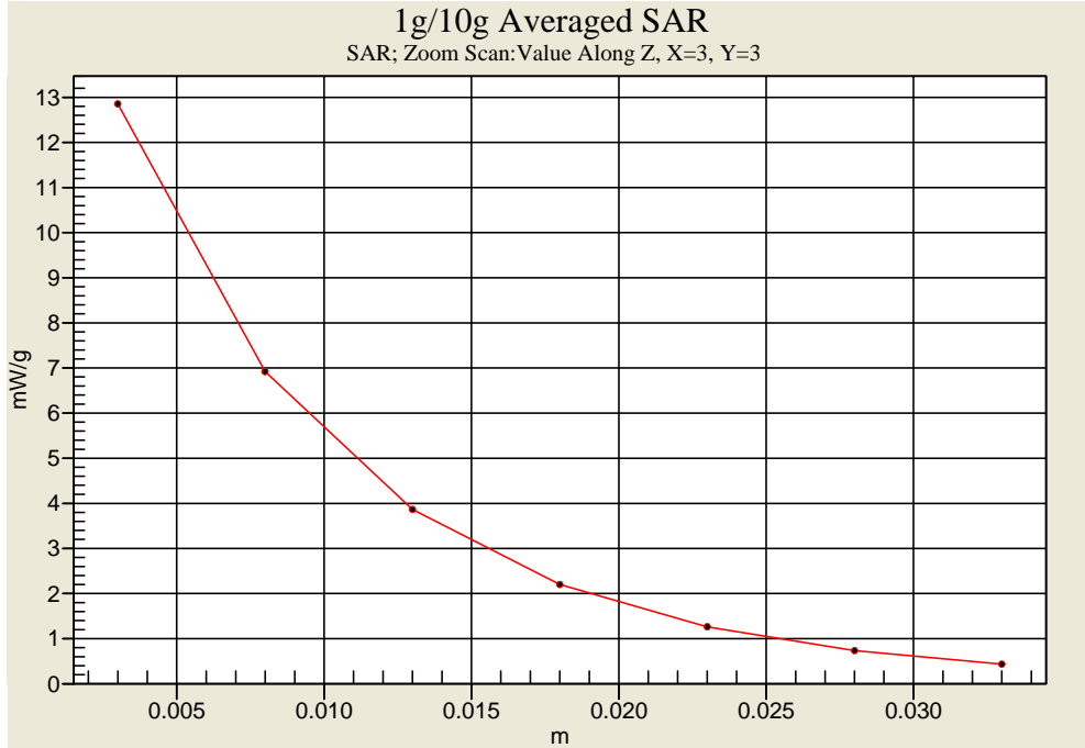
Head-Tissue-Simulating-Liquid 1900MHz(02/21/2011)
