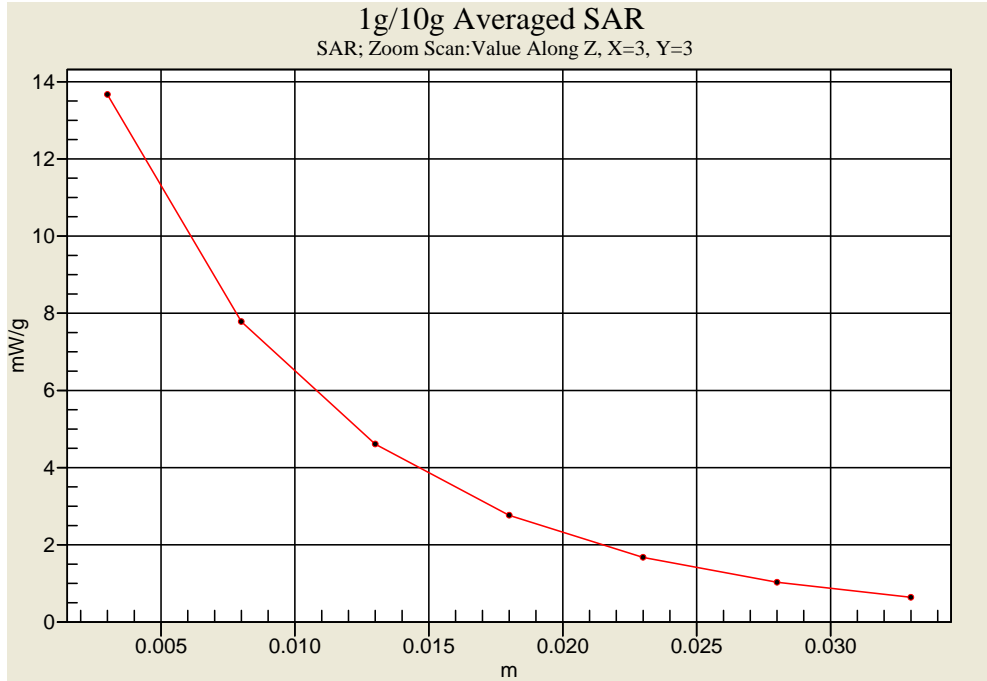
Body-Tissue-Simulating-Liquid 1900MHz(02/22/2011)
