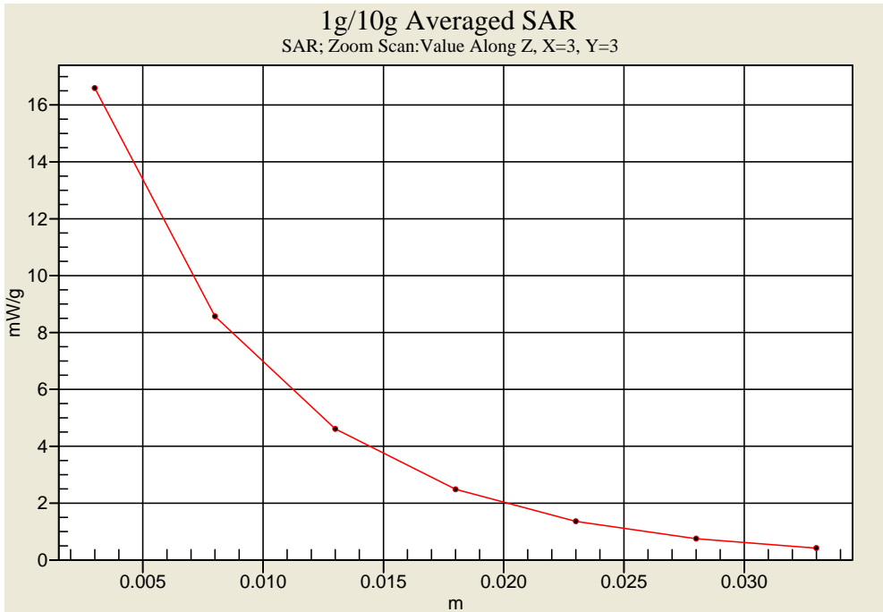
Body-Tissue-Simulating-Liquid 2450MHz(10/06/2010)
