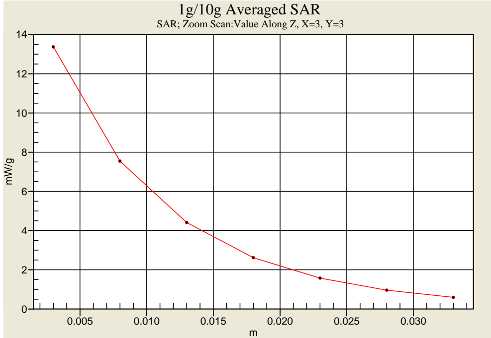
Body-Tissue-Simulating-Liquid 1900MHz(10/21/2010)
