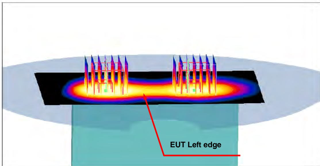
Body SAR Test Setup (Flat Section)
