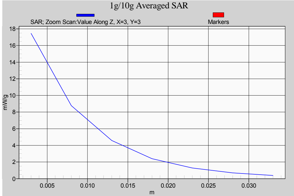
Body-Tissue-Simulating-Liquid 2450MHz_08/04/2010
