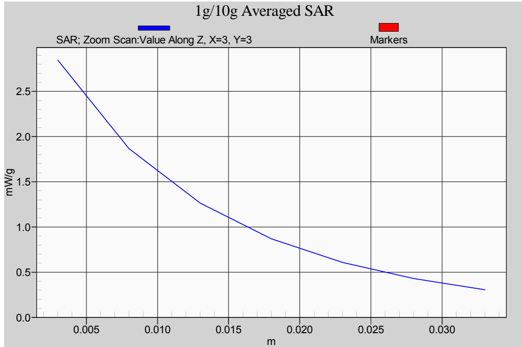
Head-Tissue-Simulating-Liquid 835MHz_08/02/2010
