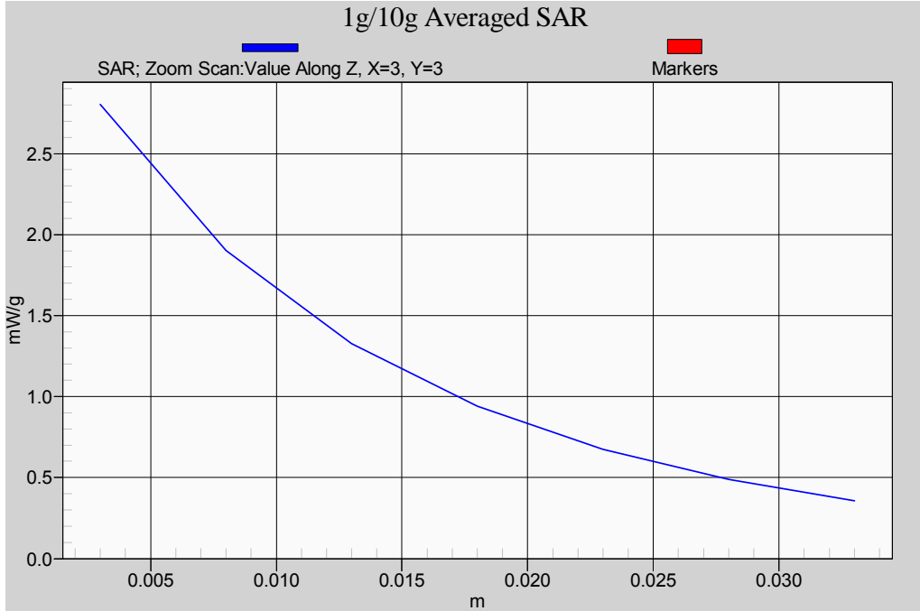
Body-Tissue-Simulating-Liquid 835MHz_07/30/2010
