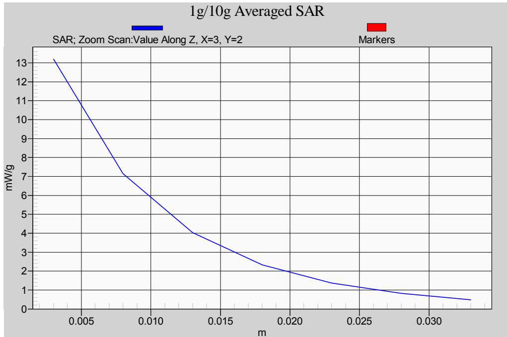
Head-Tissue-Simulating-Liquid 1900MHz_08/03/2010
