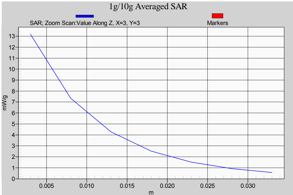
Body-Tissue-Simulating-Liquid 1900MHz_08/02/2010
