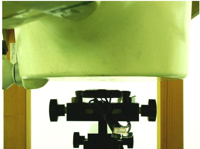
Bottom of the DUT with Phantom 1.5 cm Gap for Sample 1
