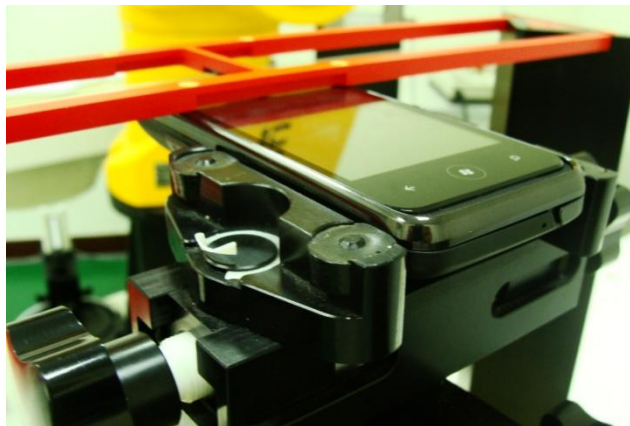
Right Side View (DUT Slide Off)
