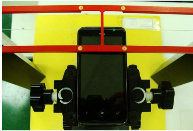
Front View (DUT Slide Off)
