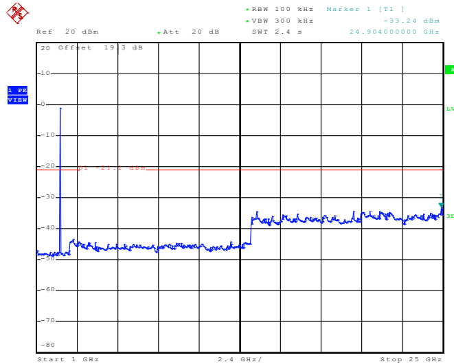
Conducted Spurious Emission Plot between 1 GHz ~ 25 GHz
