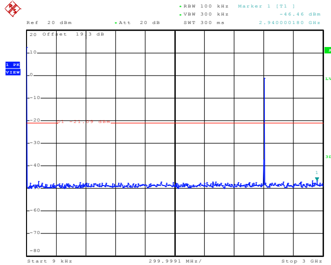
Conducted Spurious Emission Plot between 9 kHz ~ 3 GHz
