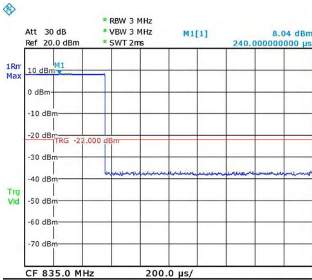
GSM Signal
