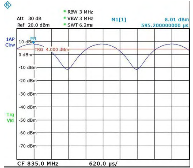
AM80%
