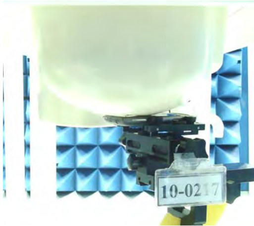
Figure 1. Right Head SAR Test Setup (Cheek)
