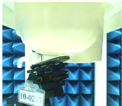
Figure 4. Left Head SAR Test Setup (Tilted)
