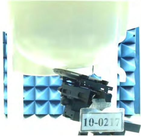
Figure 2. Right Head SAR Test Setup (Tilted)
