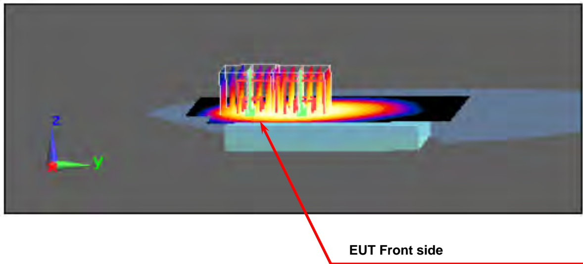
Figure 5. Body SAR Test Setup (Flat Section)
