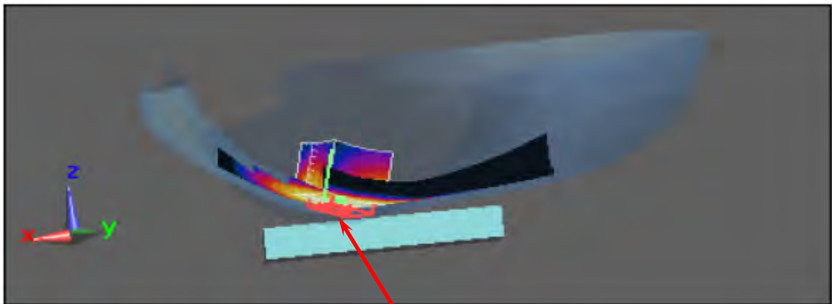
Figure 3. Left Head SAR Test Setup (Cheek)
