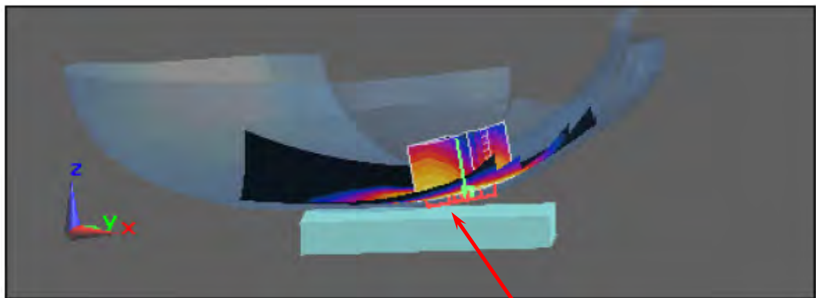
Figure 1. Right Head SAR Test Setup (Cheek)
