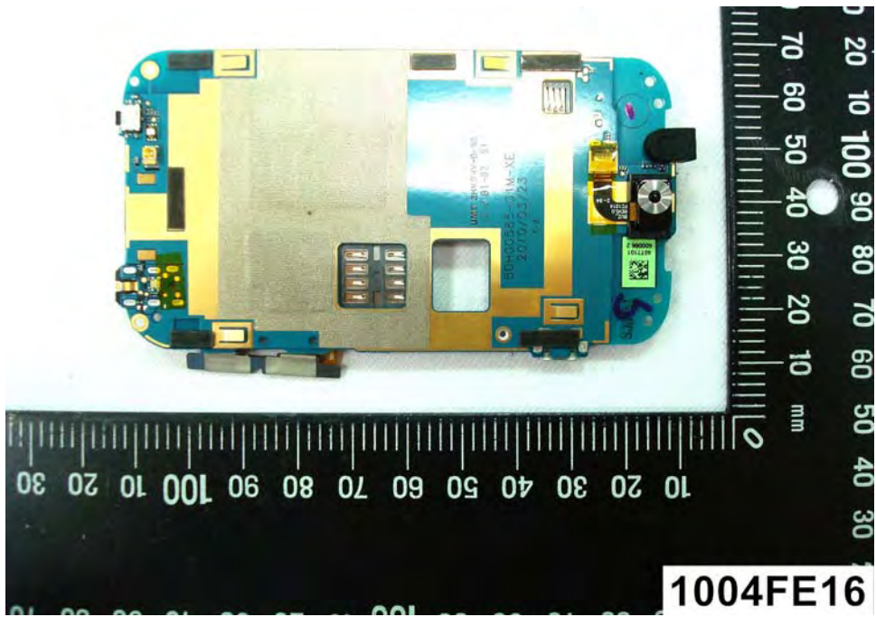
(14)EUT Photo
