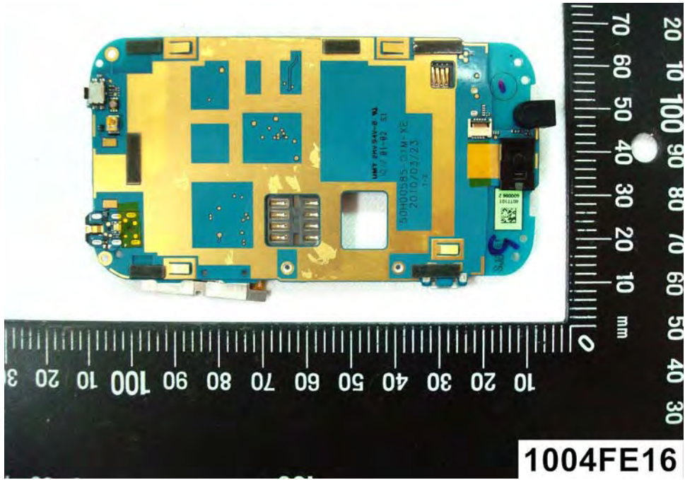
(15)EUT Photo
