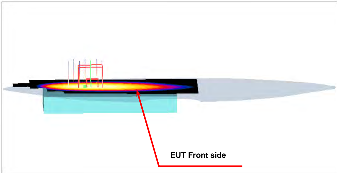
Body SAR Test Setup (Flat Section)_Open
