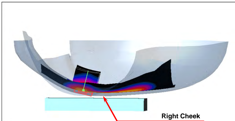
Right Head SAR Test Setup (Cheek)_Close
