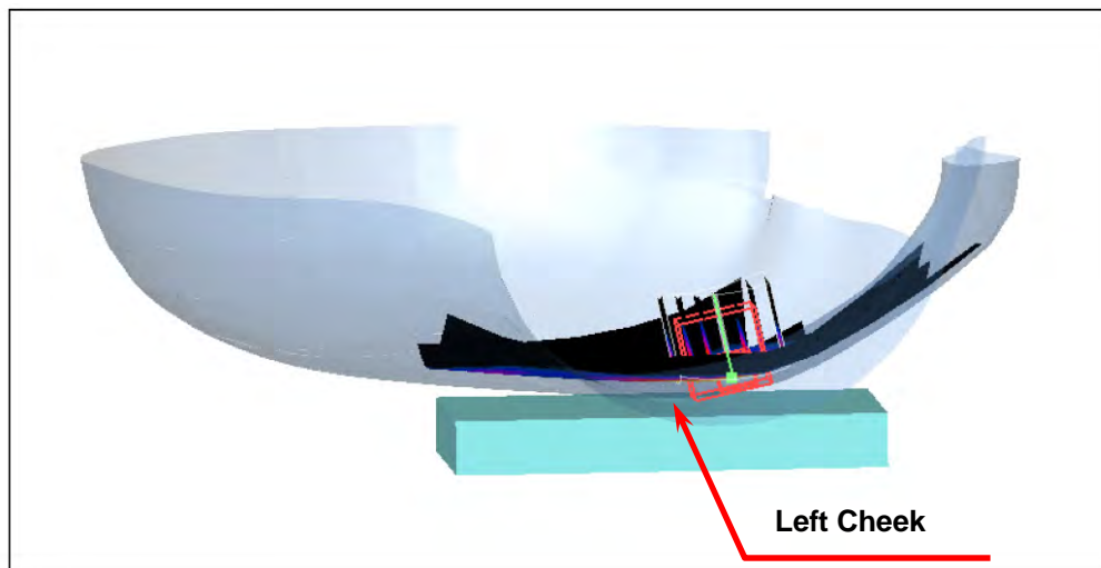
Left Head SAR Test Setup (Cheek)_Close
