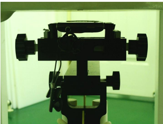
Face of the DUT with Phantom 1.5 cm Gap (With Earphone 3)
