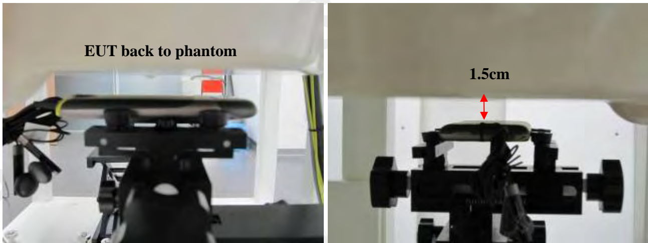
Fig.9 Body worn- EUT back to flat phantom and distance between flat phantom and mobile phone is 1.5 cm with headset
