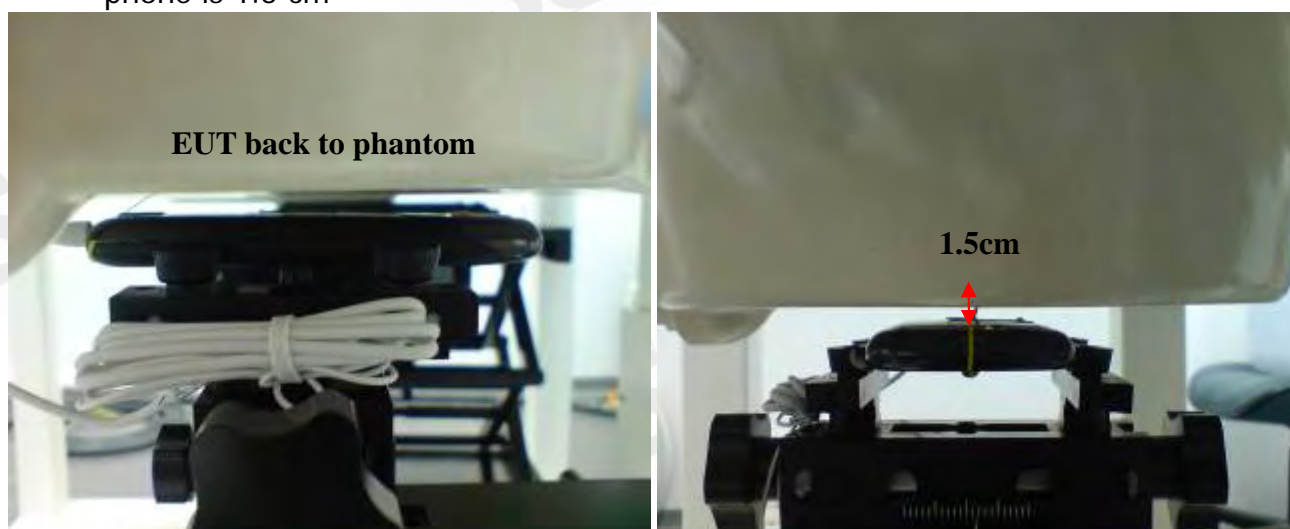
Fig.9 Body worn- EUT back to flat phantom and distance between flat phantom and mobile phone is 1.5 cm with headset
