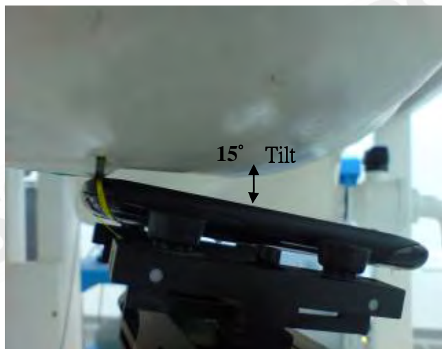
Fig.4 Right Head Section / Ear-Tilt Position(15°)
