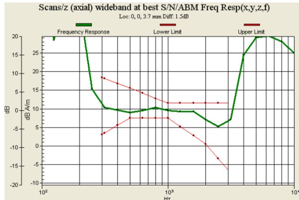
Fig. 9.7 GSM1900 Ch661 for Sample A
