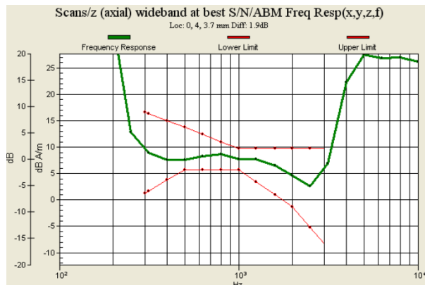
Fig. 9.9 WCDMA Band V Ch4132 for Sample A
