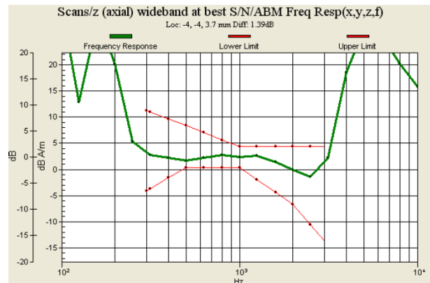
Fig. 9.10 WCDMA Band V Ch4182 for Sample A
