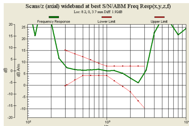
Fig. 9.14 WCDMA Band II Ch9400 for Sample A
