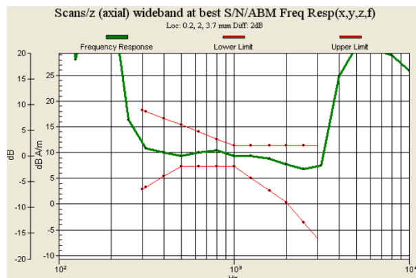
Fig. 9.3 GSM850 Ch189 for Sample B
