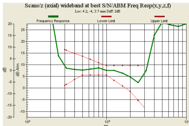
Fig. 9.11 WCDMA Band V Ch4233 for Sample A
