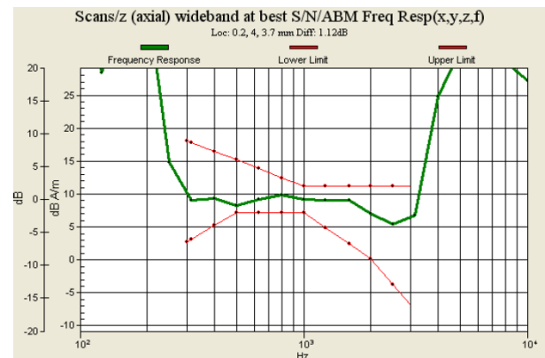
Fig. 9.2 GSM850 Ch189 for Sample A
