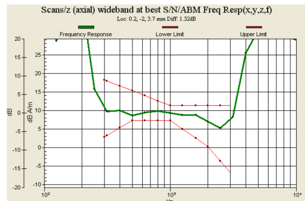
Fig. 9.4 GSM850 Ch251 for Sample A
