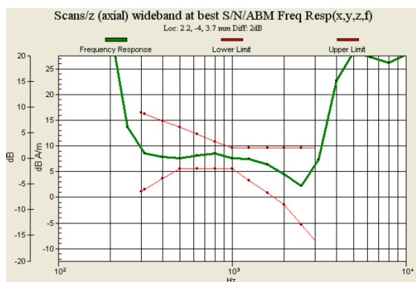
Fig. 9.15 WCDMA Band II Ch9538 for Sample A
