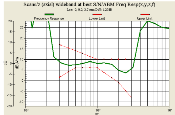
Fig. 9.8 GSM1900 Ch810 for Sample A
