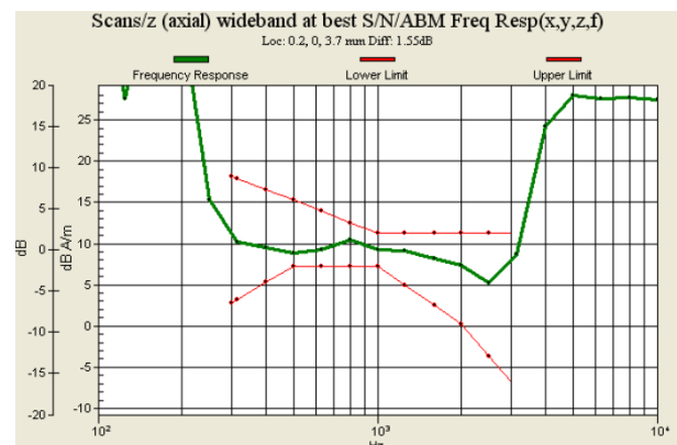
Fig. 9.6 GSM1900 Ch512 for Sample B
