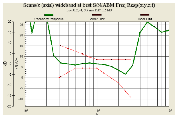
Fig. 9.12 WCDMA Band V Ch4233 for Sample B
